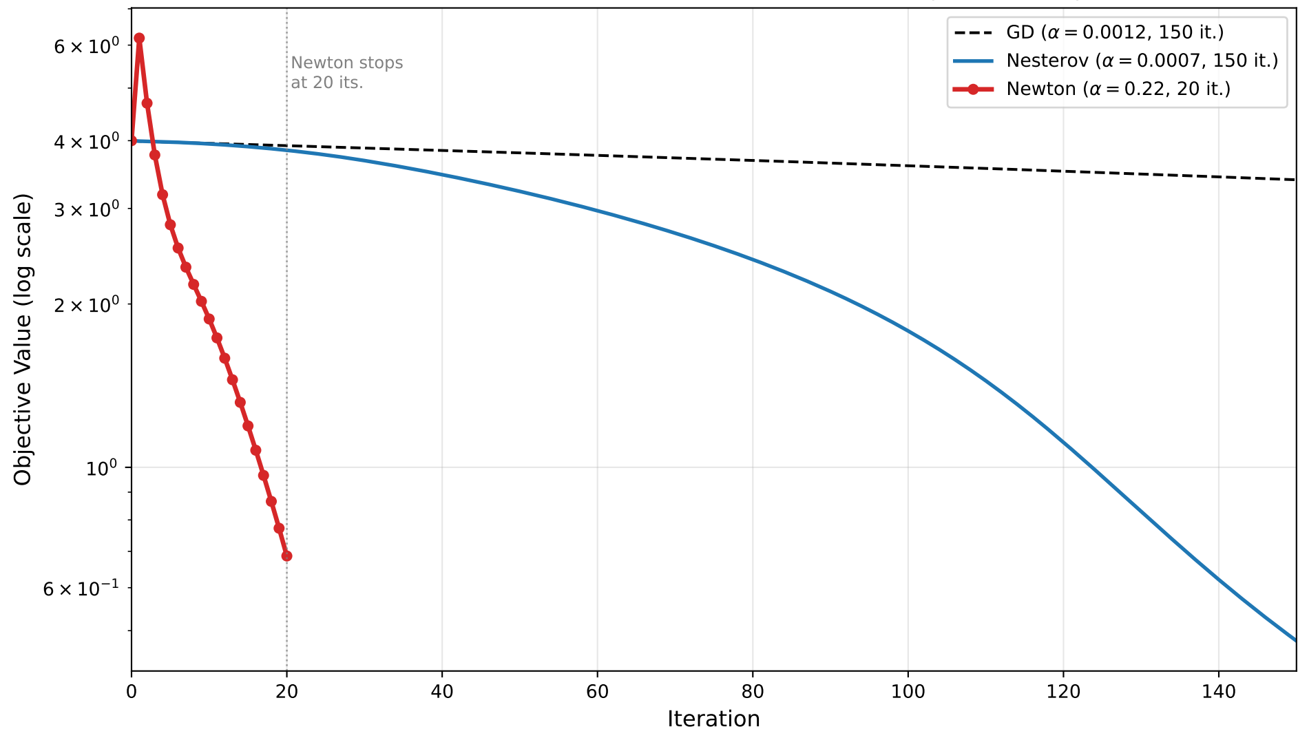
Newton vs First-Order Methods on Benchmark C (Rosenbrock)
