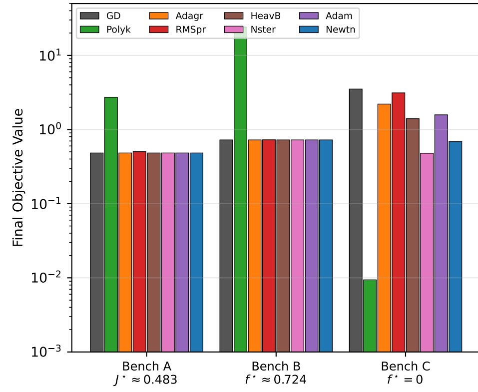
All Methods, All Benchmarks (grouped by benchmark)
