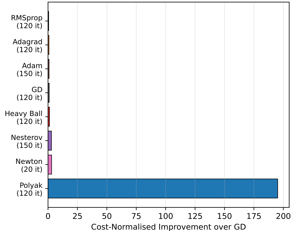
Cost-Efficiency: improvement/GD divided by relative compute cost
