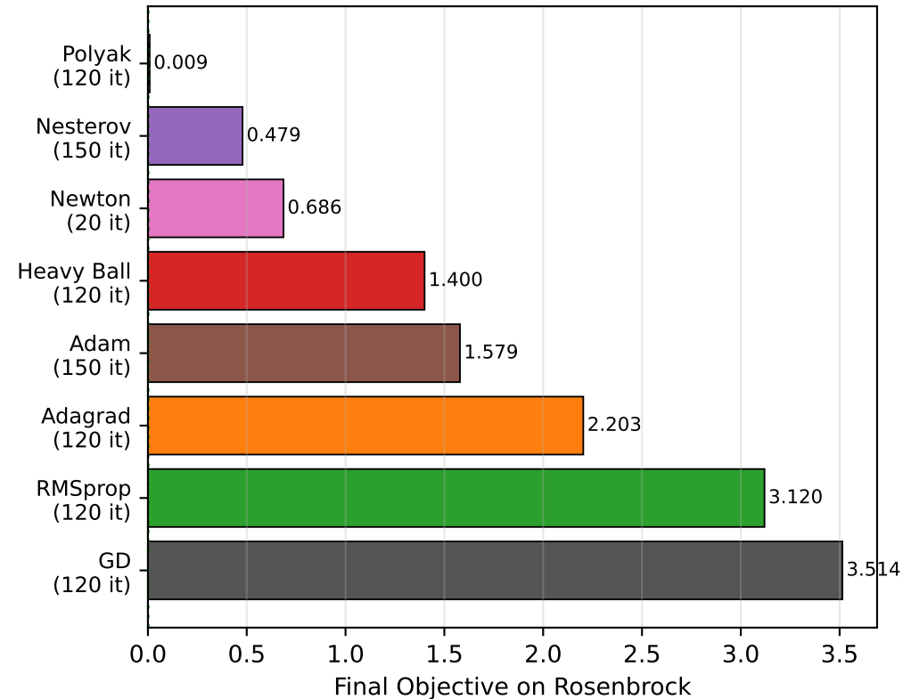
Method Ranking: Rosenbrock (lower is better)
