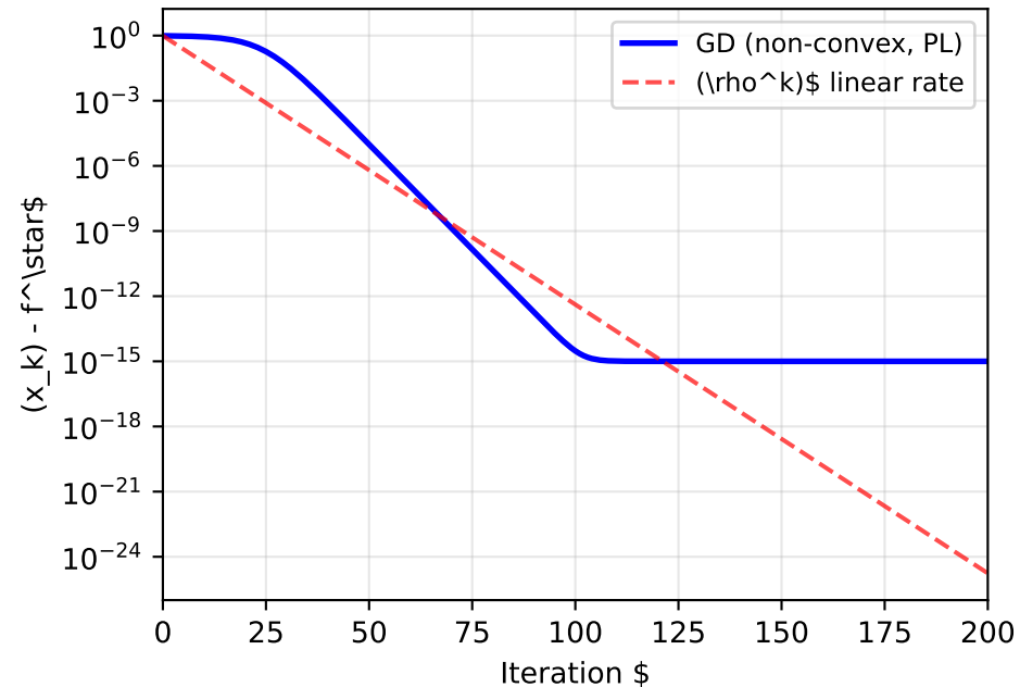
GD on PL function: (a,b)=(ab-1)^2 (non-convex, multiple global minima)
