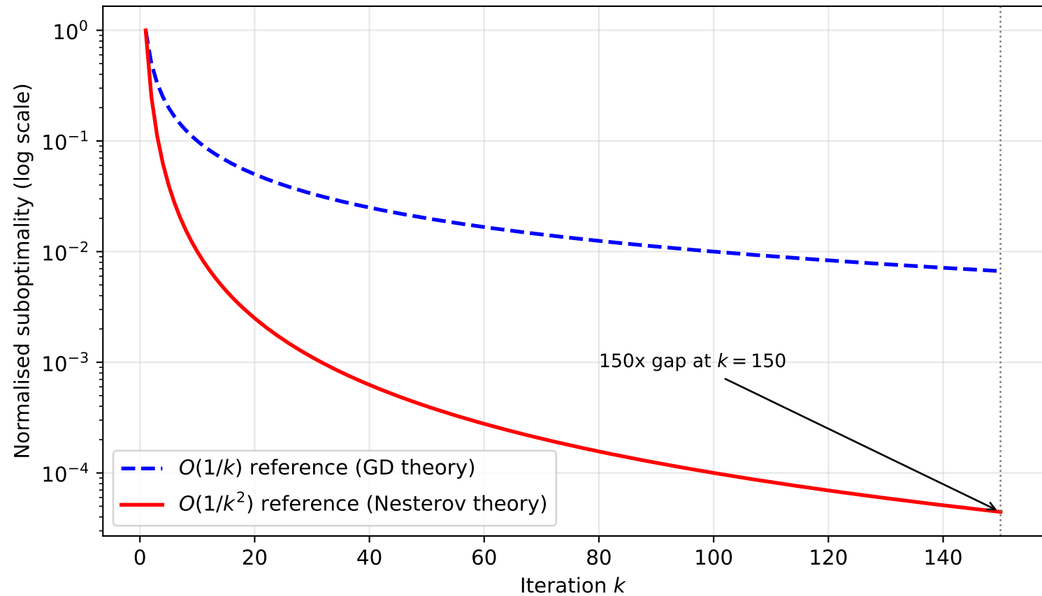
Theoretical Convergence Rates: O(1/k) vs O(1/k^2)
