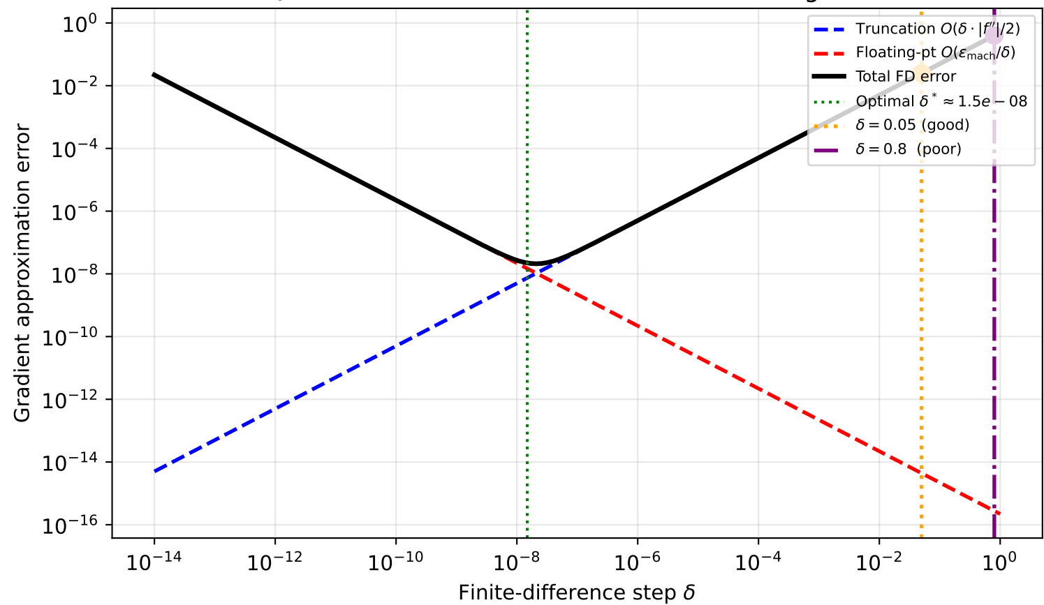
Q4: FD Error Trade-off: Truncation vs Floating-Point
