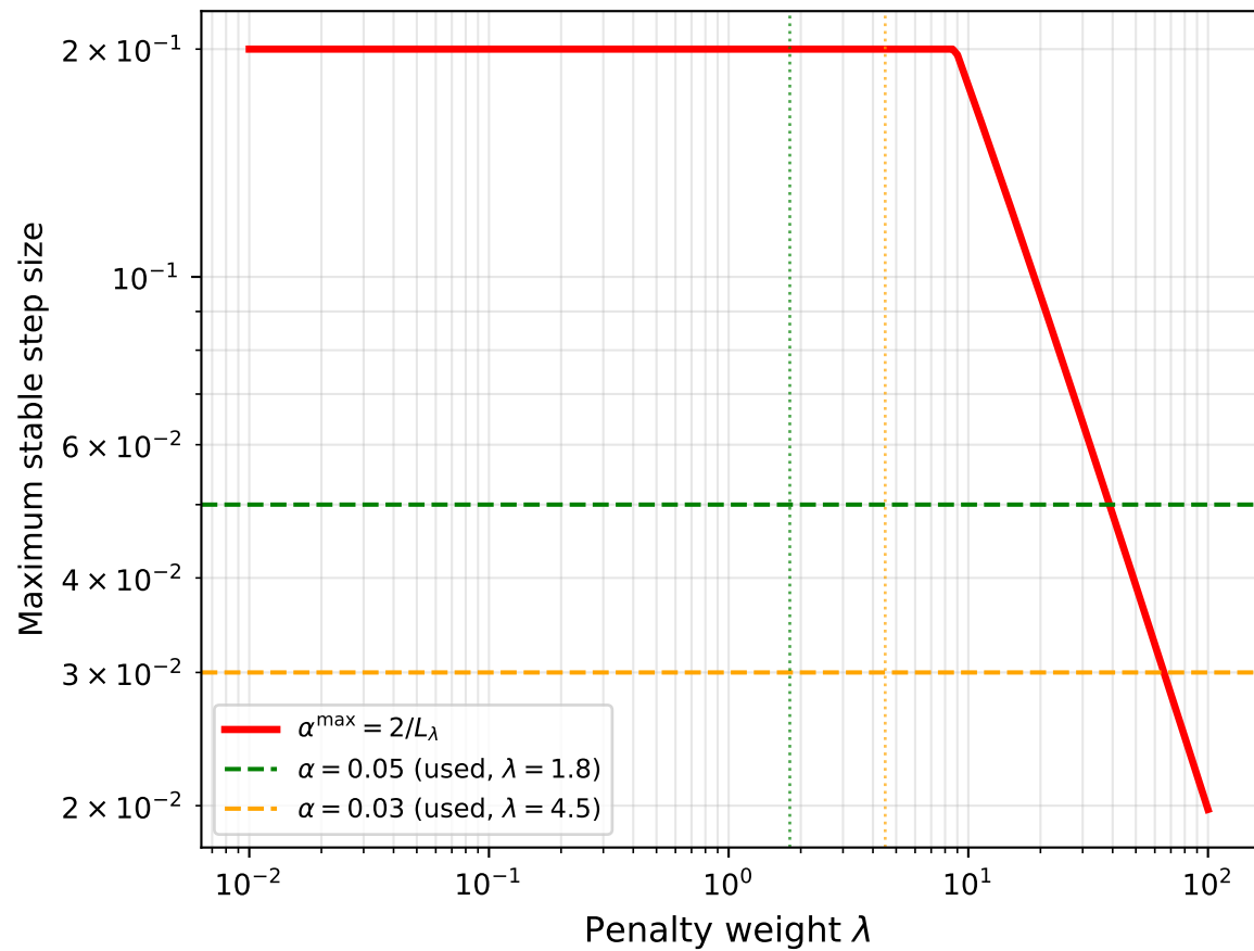
Maximum stable step size vs. \lambda
