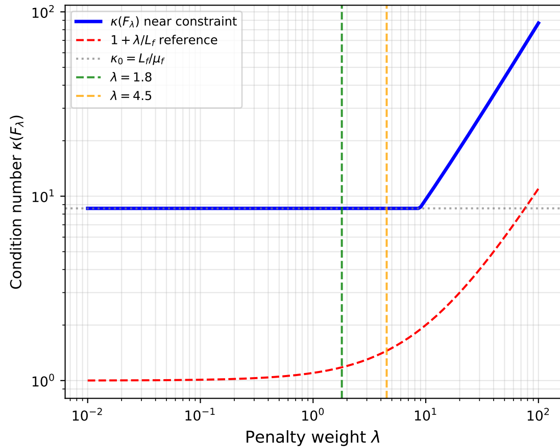
Conditioning of penalised objective vs. \lambda
