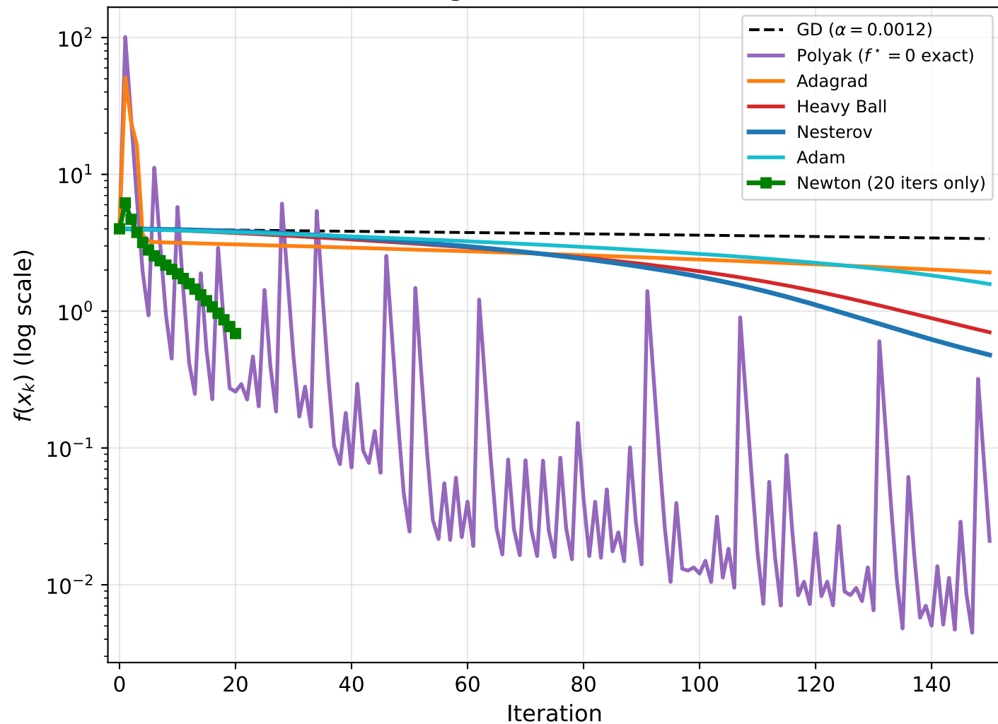
All Methods: Convergence on Rosenbrock (Benchmark C)
