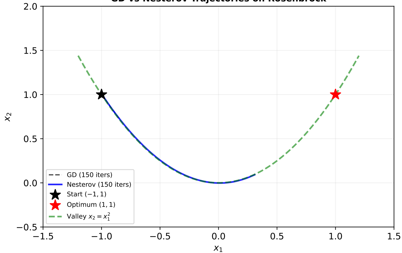
GD vs Nesterov Trajectories on Rosenbrock
