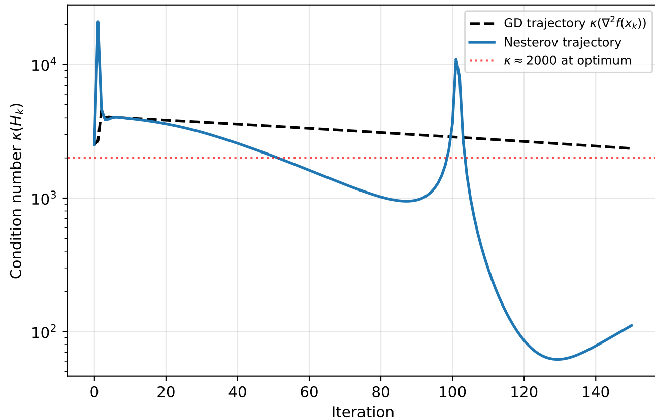
Hessian Condition Number Along Trajectory (Benchmark C: Rosenbrock)
