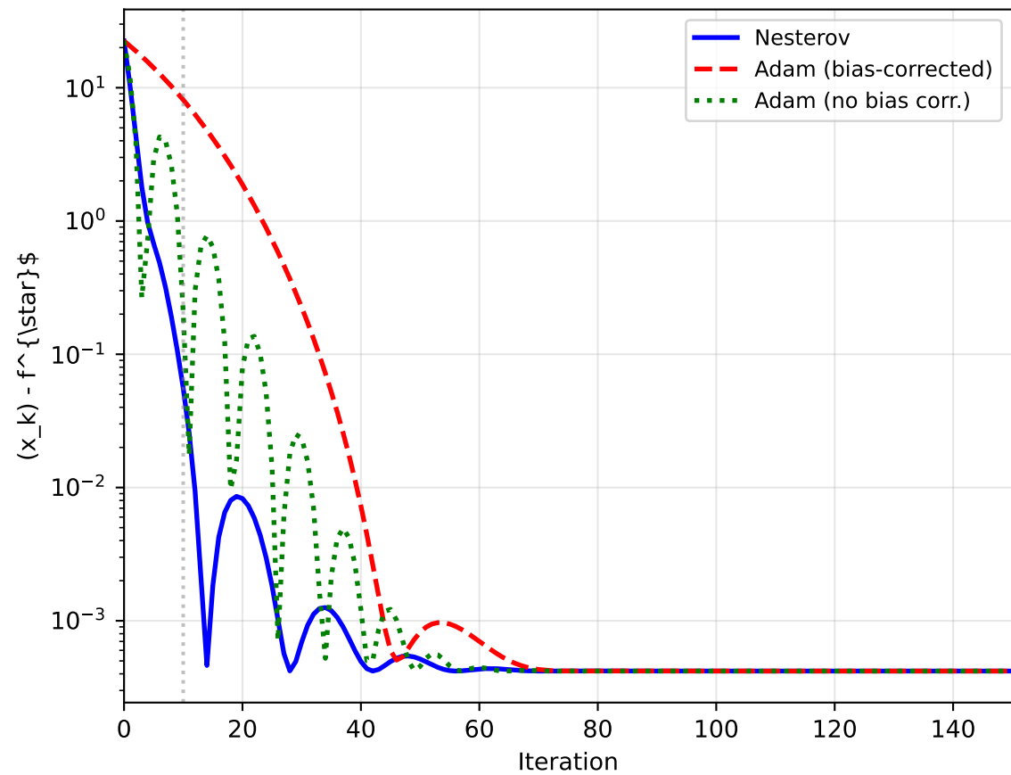
Nesterov vs Adam: Benchmark B
