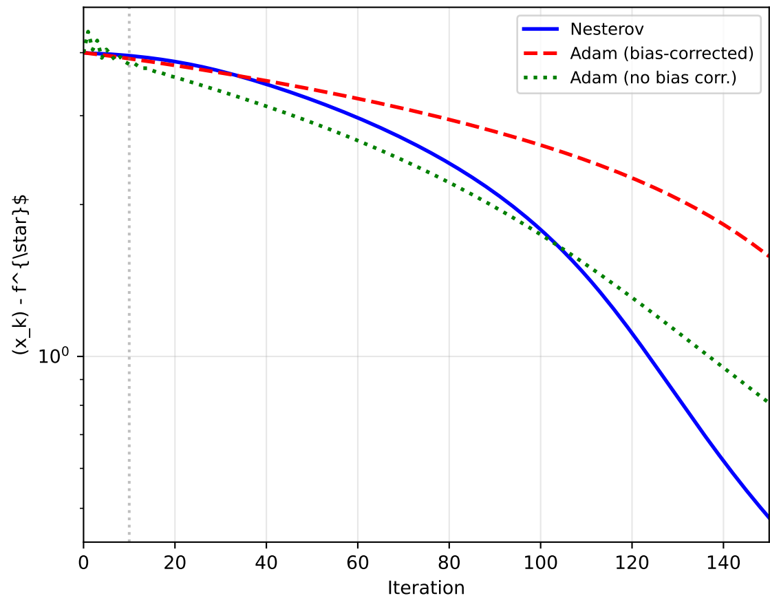
Nesterov vs Adam: Benchmark C (Rosenbrock)
