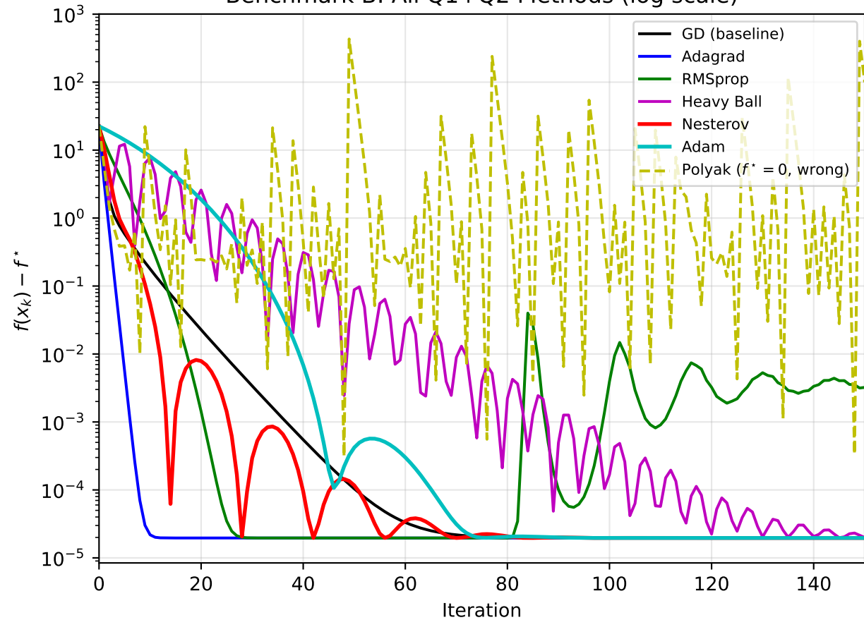
Benchmark B: All Q1+Q2 Methods (log scale)
