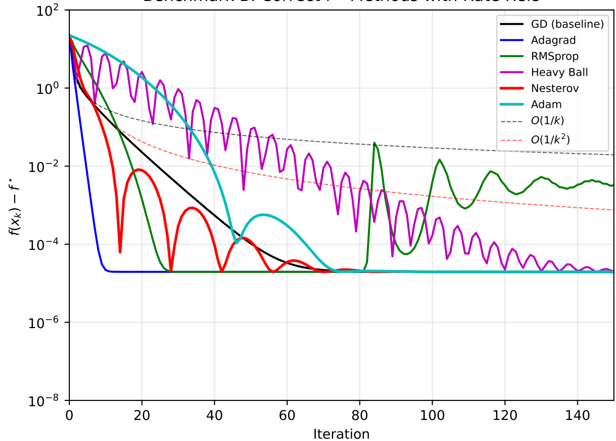
Benchmark B: Correct- f^* Methods with Rate Refs
