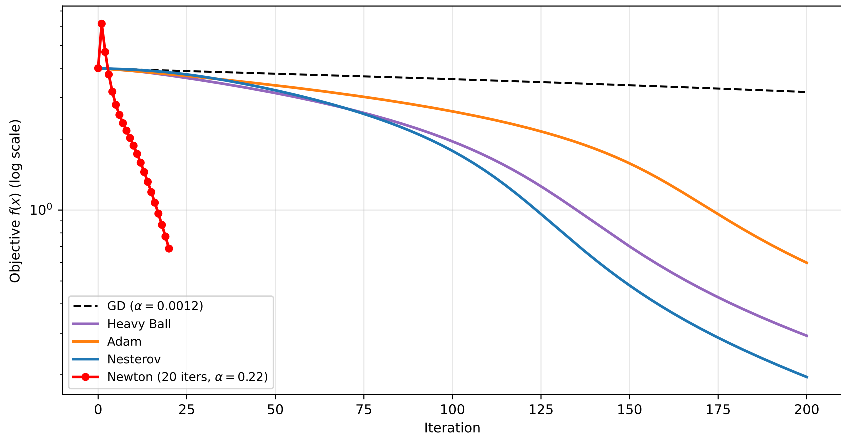
All Methods on Benchmark C (Rosenbrock) — 200 Iterations
