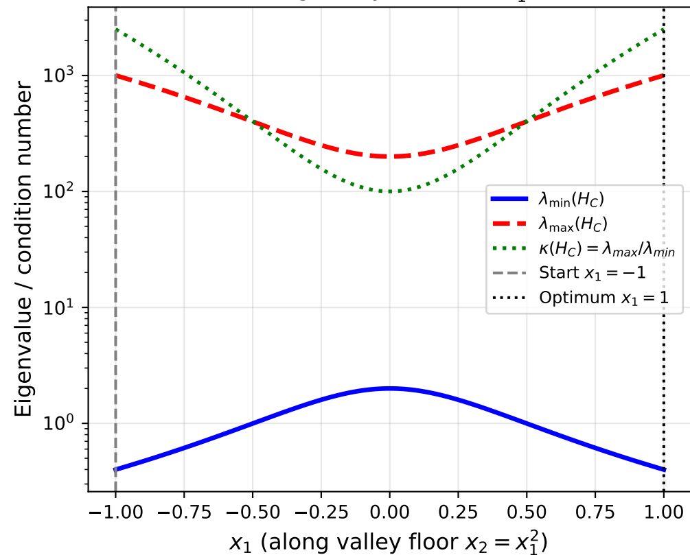
Benchmark C: Rosenbrock Hessian along Valley Floor x_2 = x_1^2
