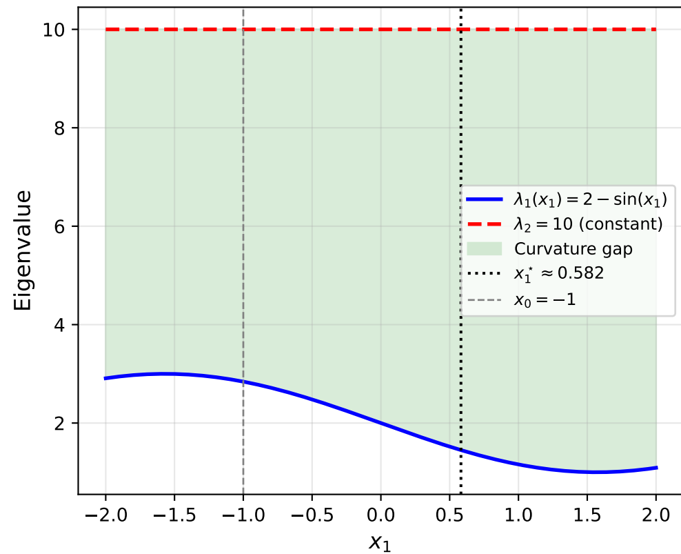
Benchmark B: Hessian Eigenvalues H_B(x) = \text{diag}(2 - \sin(x_1), 10)
