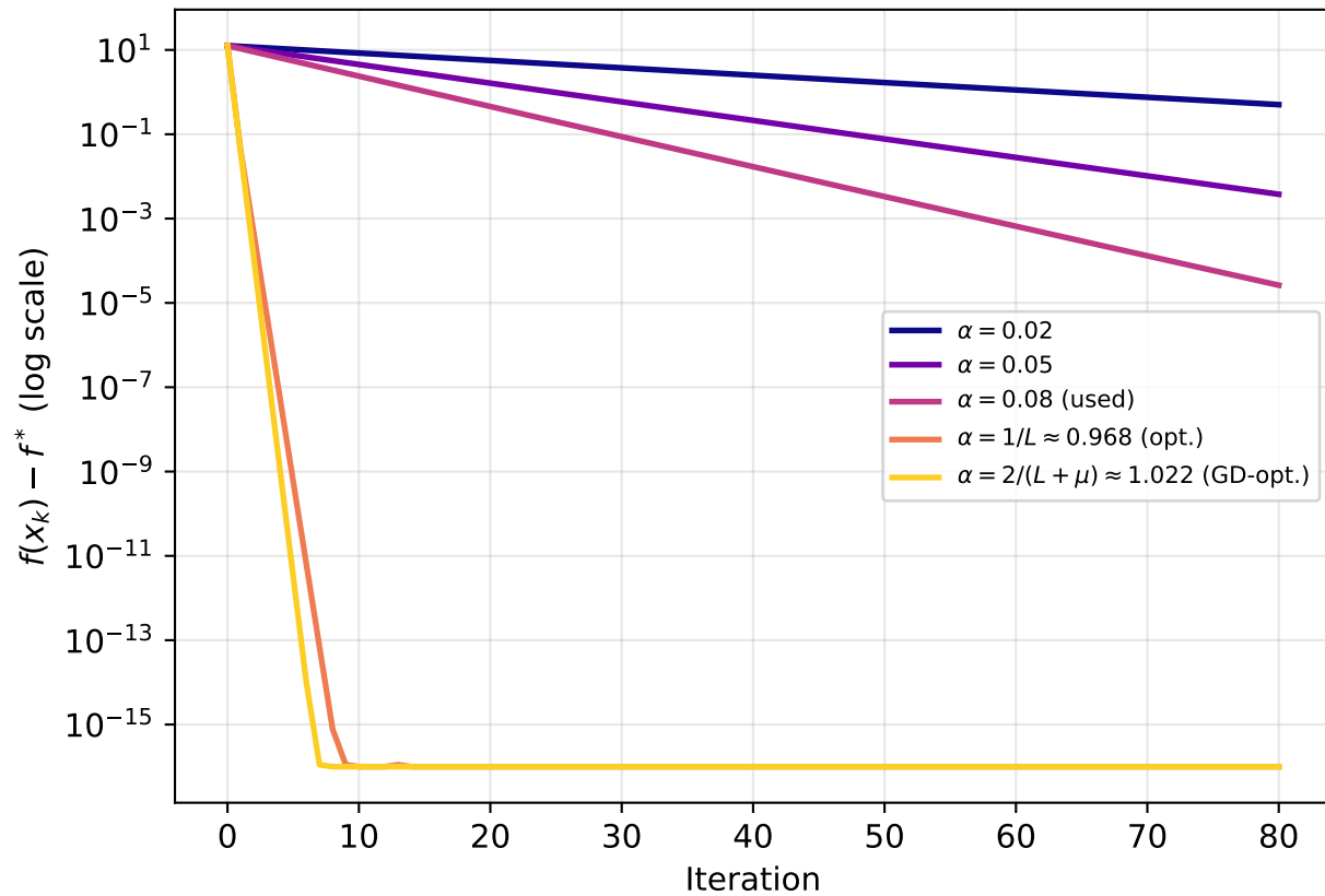
Q1: Effect of Step Size on GD — Benchmark A (Linear Regression, \kappa \approx 1.12 )
