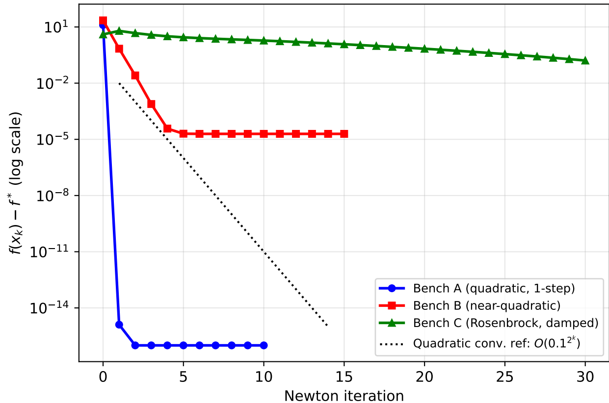
Q3: Newton's Method Convergence Speed vs Function Convexity/Quadraticity
