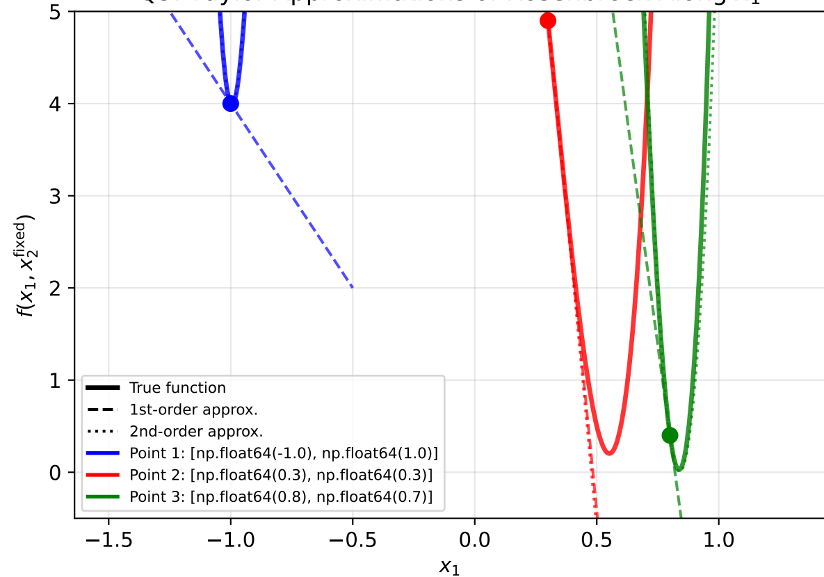
Q3: Taylor Approximations of Rosenbrock Along x_1
