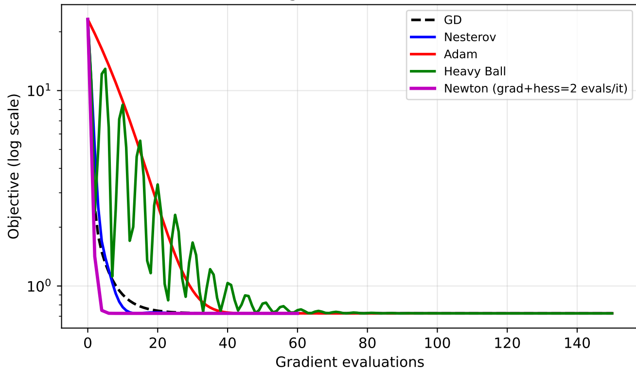
Benchmark B: Convergence per Gradient Evaluation (Newton counts gradient + Hessian as 2 evals)
