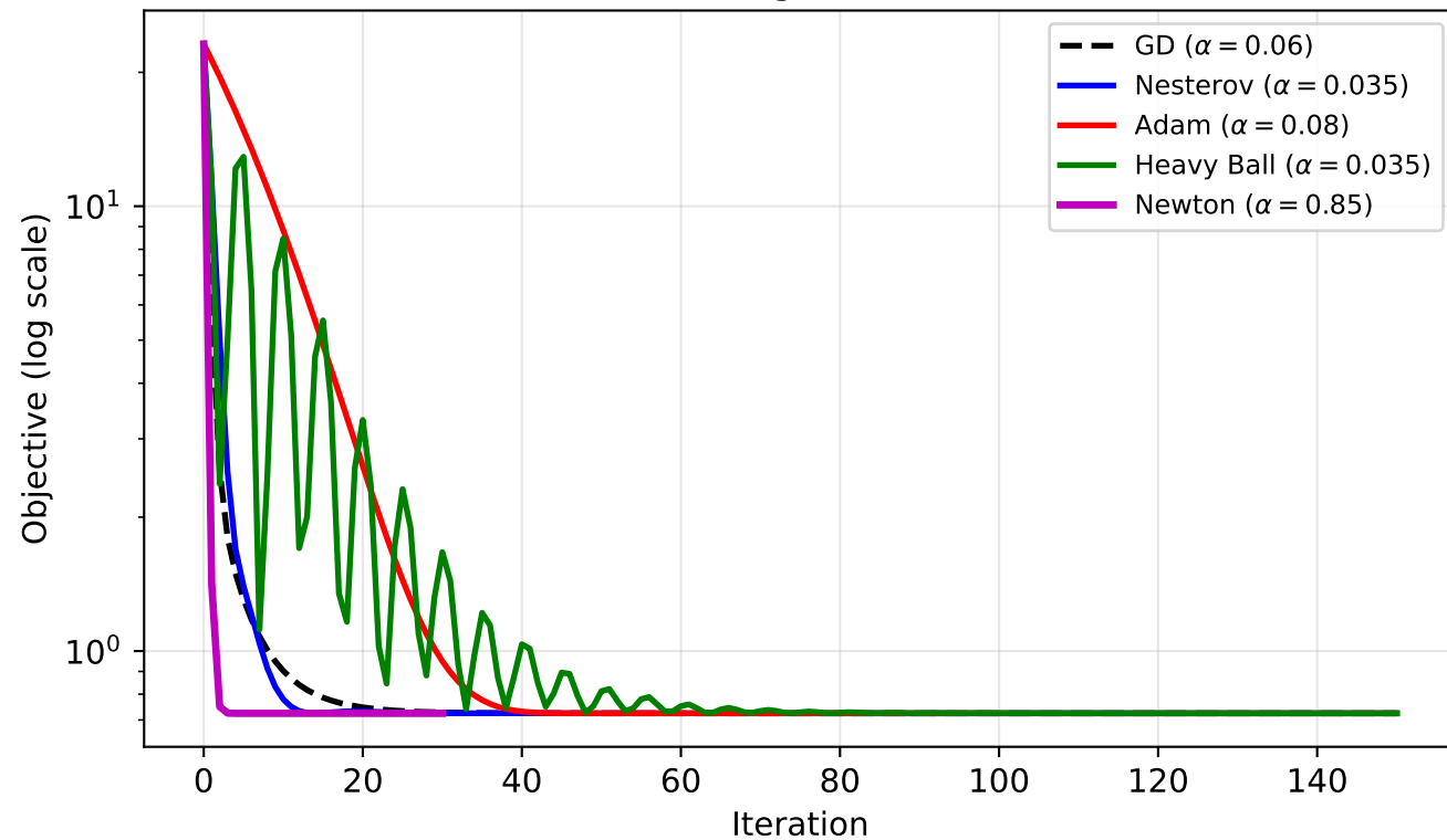
Benchmark B: Convergence vs Iteration Count
