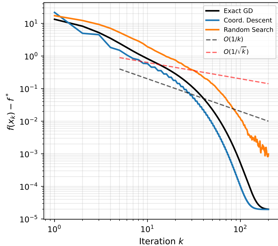
Log-log Rate Verification
