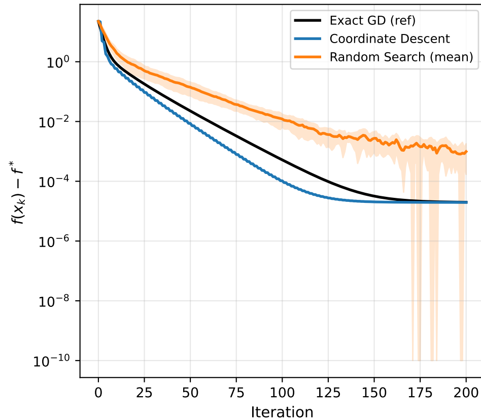
Convergence Comparison (Benchmark B, 200 iters)
