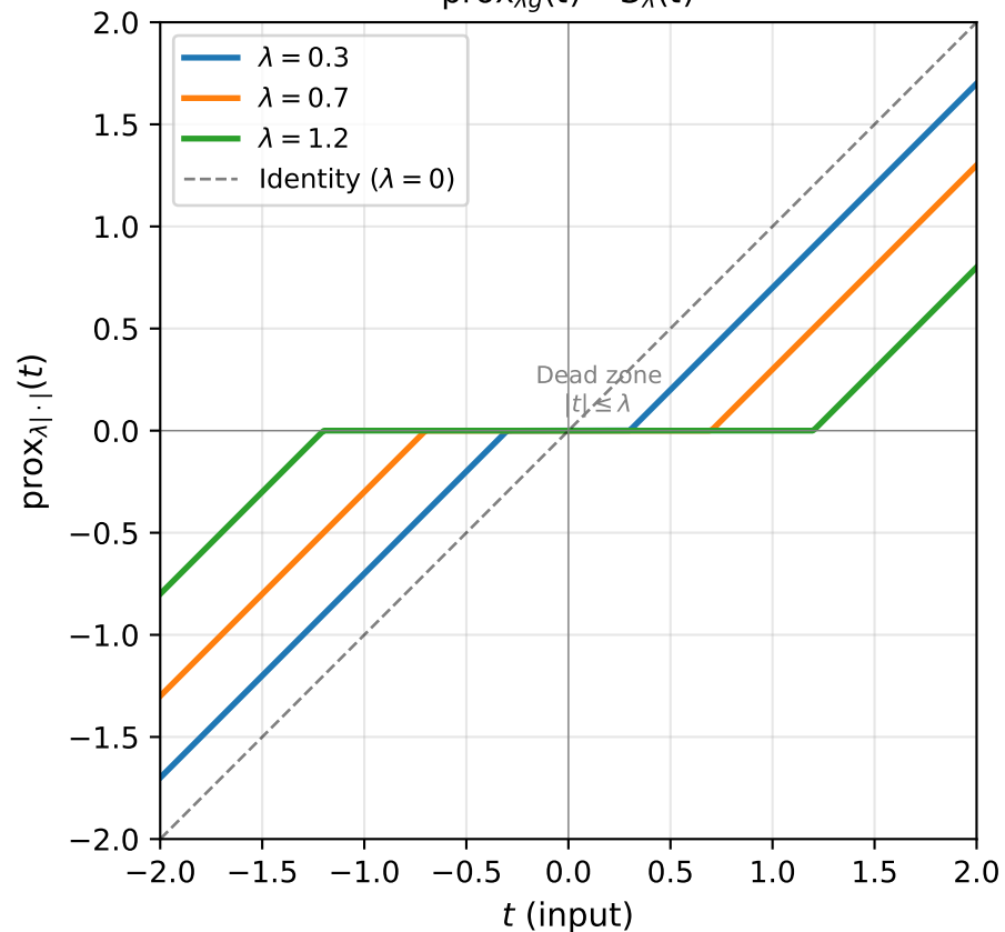
Soft Thresholding (Prox of \ell_1 ) \text{prox}_{\lambda g}(t) = S_\lambda(t)
