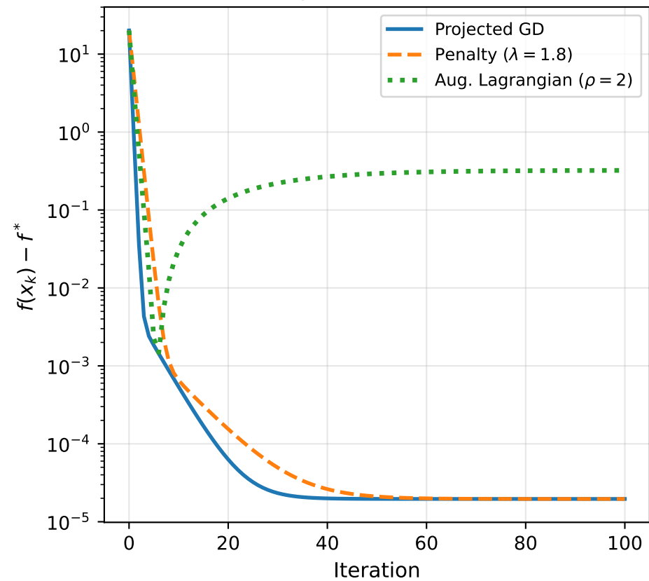
Constrained Methods: Objective Gap (Q5 problem, 100 iters)
