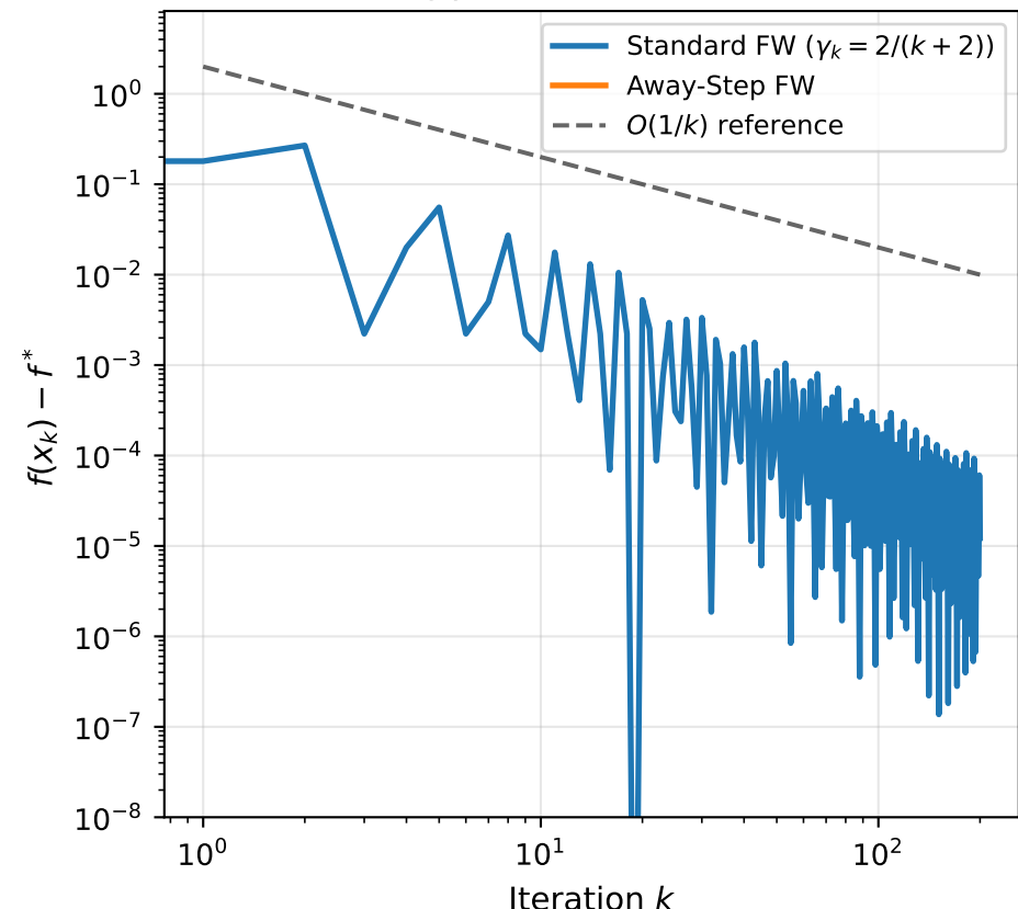
Standard FW vs Away-Step FW (Strongly convex, box constraint)
