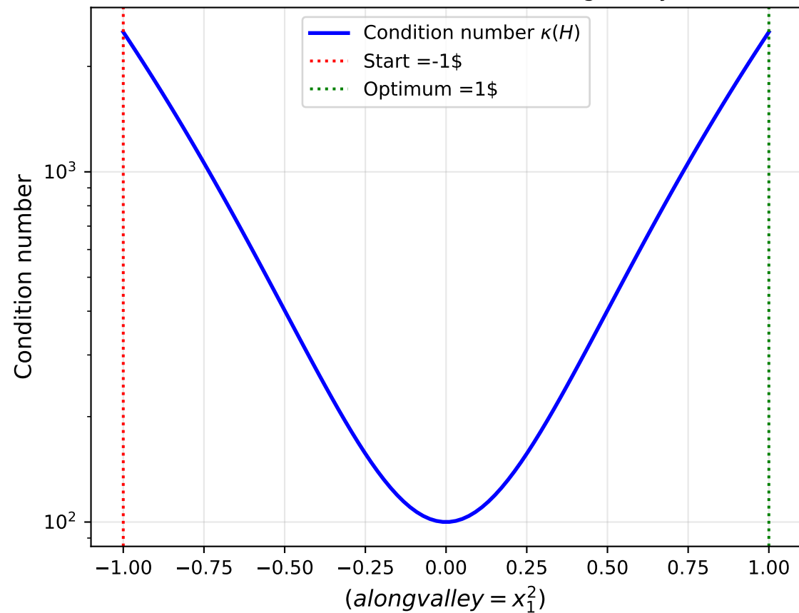
Hessian Condition Number Along Valley
