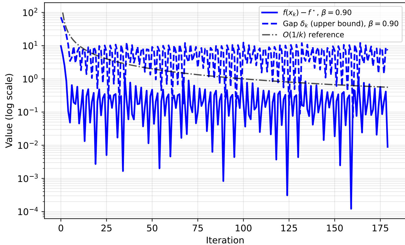
Gap \delta_k \geq f(x_k) - f^* (Certificate)
