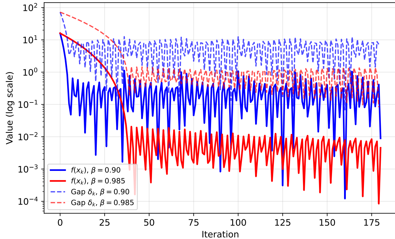
Frank--Wolfe: Objective and Gap Certificate
