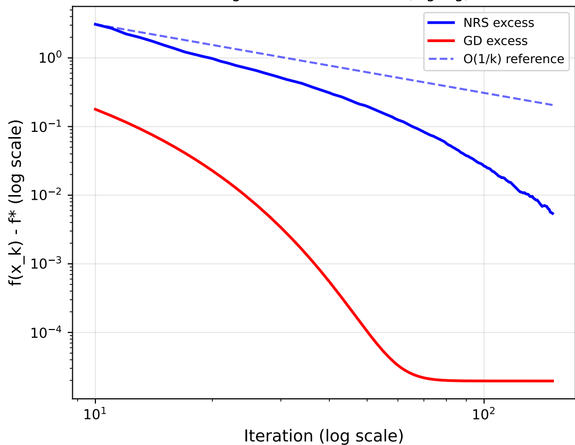
Convergence rate verification (log-log)
