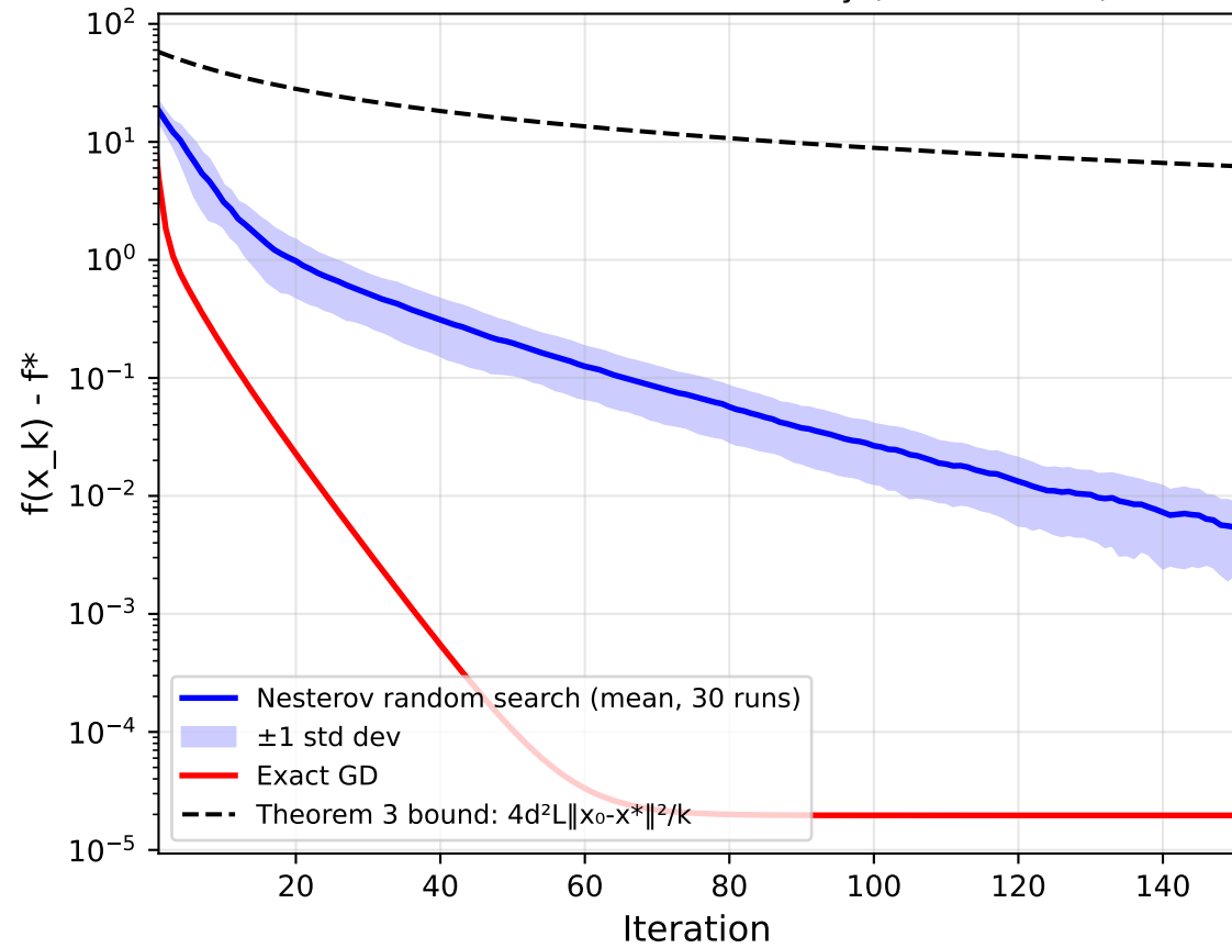
Nesterov Random Search vs Theory (Benchmark B)
