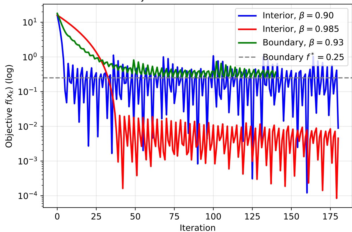
Objective Value vs Iteration
