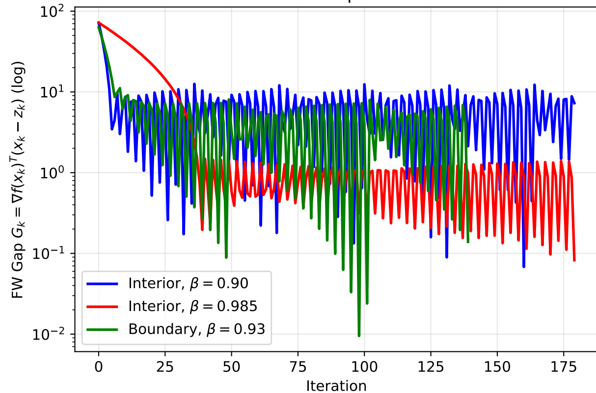
Frank--Wolfe Gap vs Iteration
