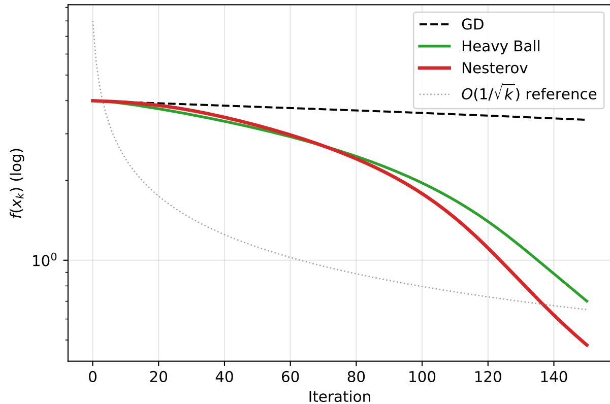
Q1/Q2: Momentum Methods on Rosenbrock
