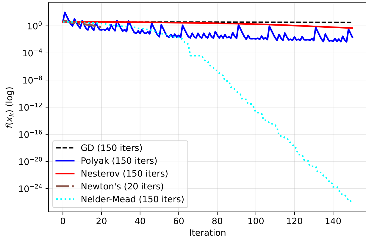
Best Methods per Category on Rosenbrock
