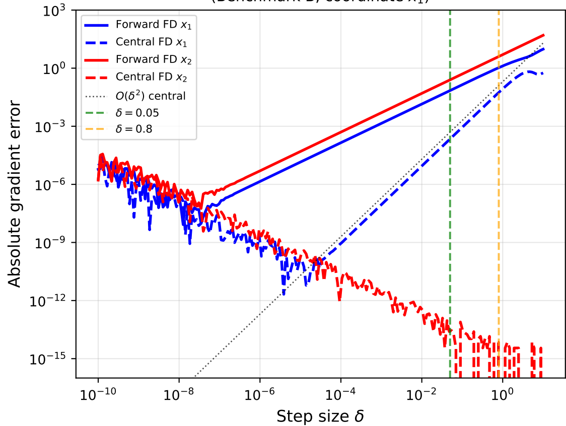
Forward vs. Central FD gradient error (Benchmark B, coordinate x_1 )
