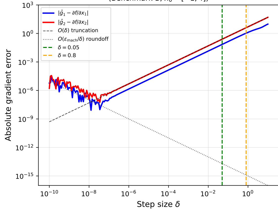
Forward FD gradient error vs. \delta (Benchmark B, x_0 = [-1, 4] )
