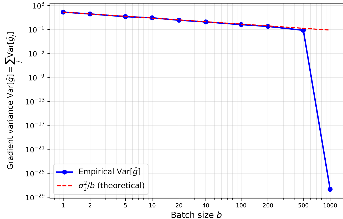
Mini-batch gradient variance vs. batch size (Benchmark A, \theta_0 = [0, 0] )
