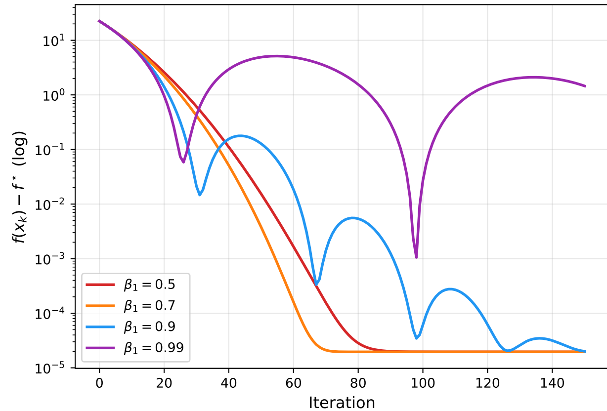
Adam: Effect of \beta_1 (First Moment Decay) (Benchmark B)
