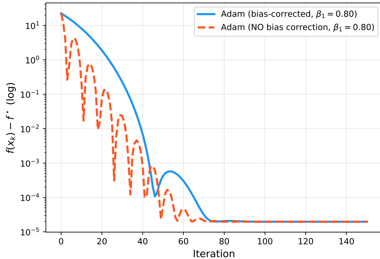
Effect of Bias Correction in Adam (Benchmark B, \alpha = 0.08 , \beta_2 = 0.999 )
