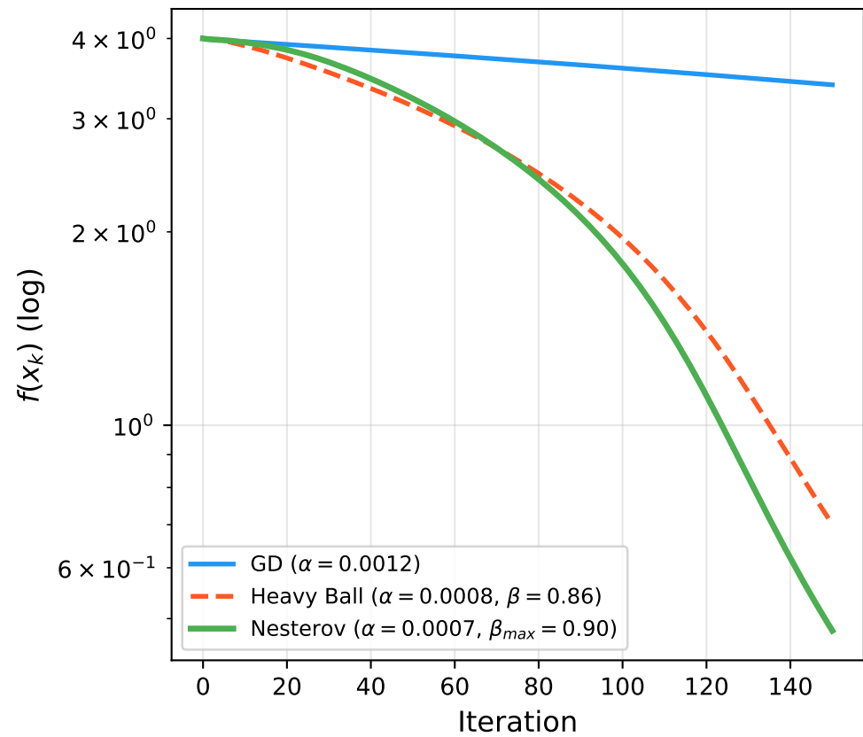
GD vs Heavy Ball vs Nesterov Rosenbrock ( f^* = 0 )
