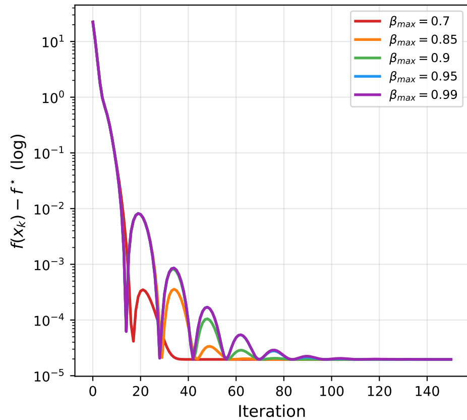
Effect of \beta_{max} on Nesterov Convergence (Benchmark B, \alpha = 0.035 )
