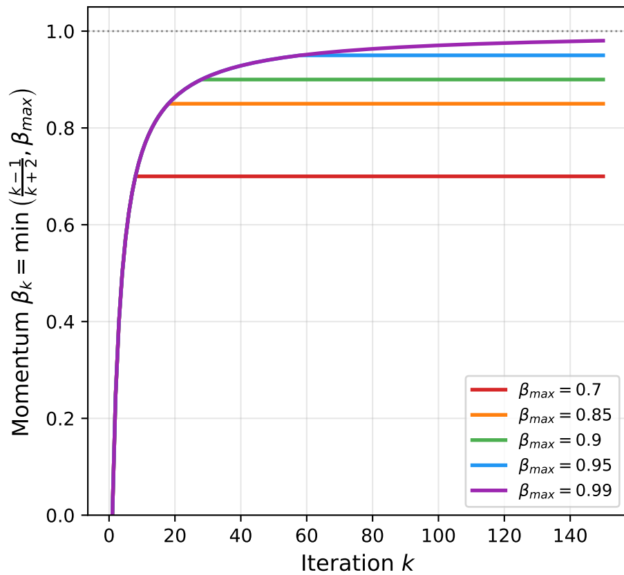
Nesterov's Adaptive Momentum Schedule \beta_k = \min((k-1)/(k+2), \beta_{max})
