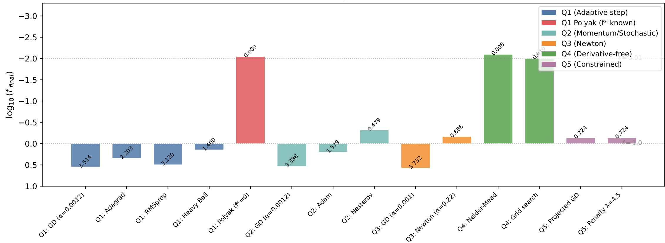
Final objective f(x_k) on Benchmark C (Rosenbrock, f^* = 0 ) log scale
