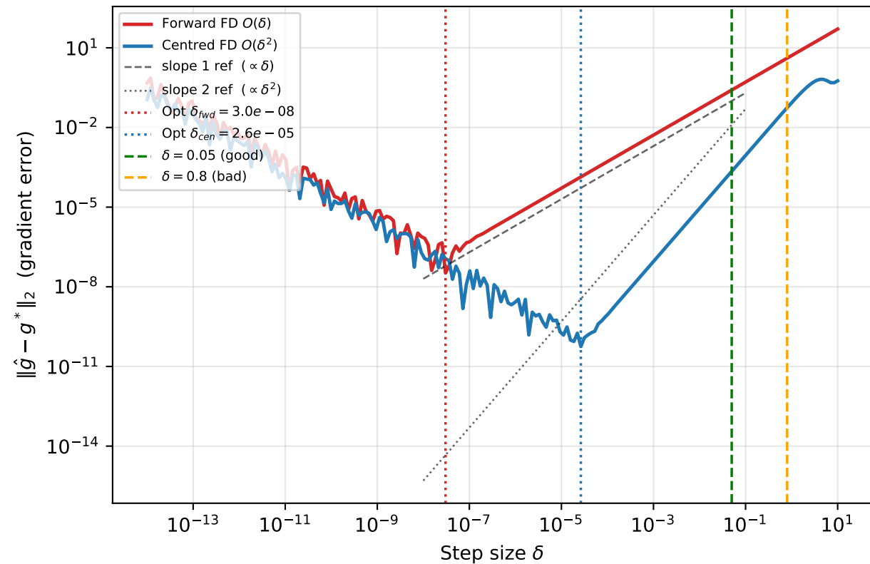
FD Error vs Step Size (Full Range)
