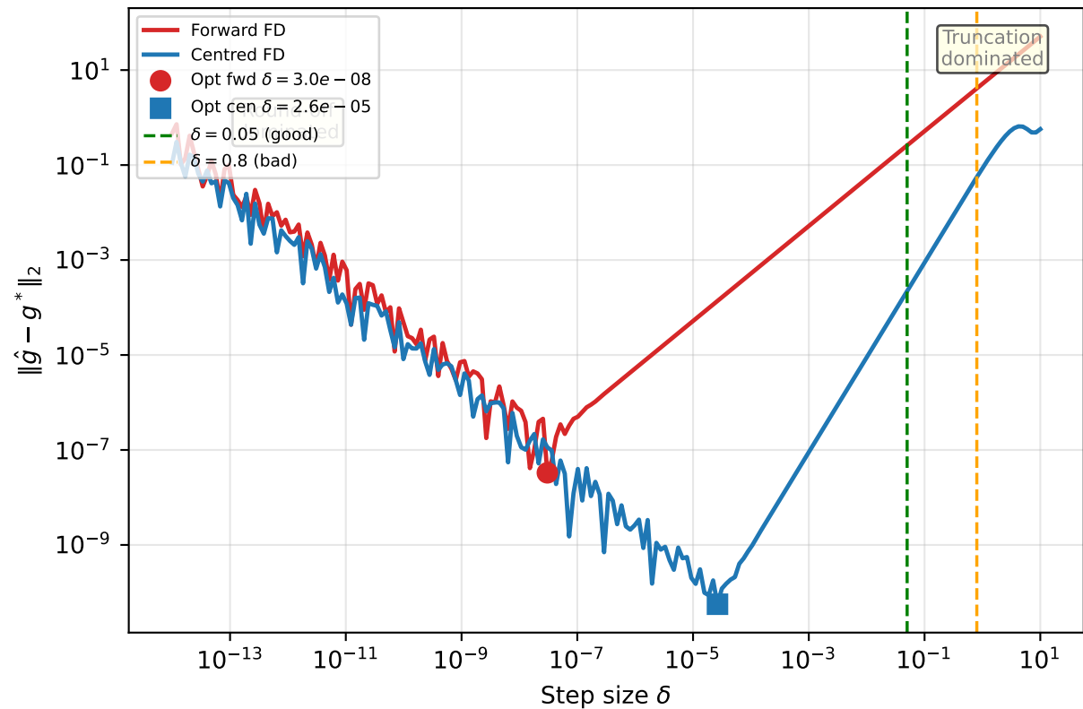
U-Shape: Truncation vs Round-off Error
