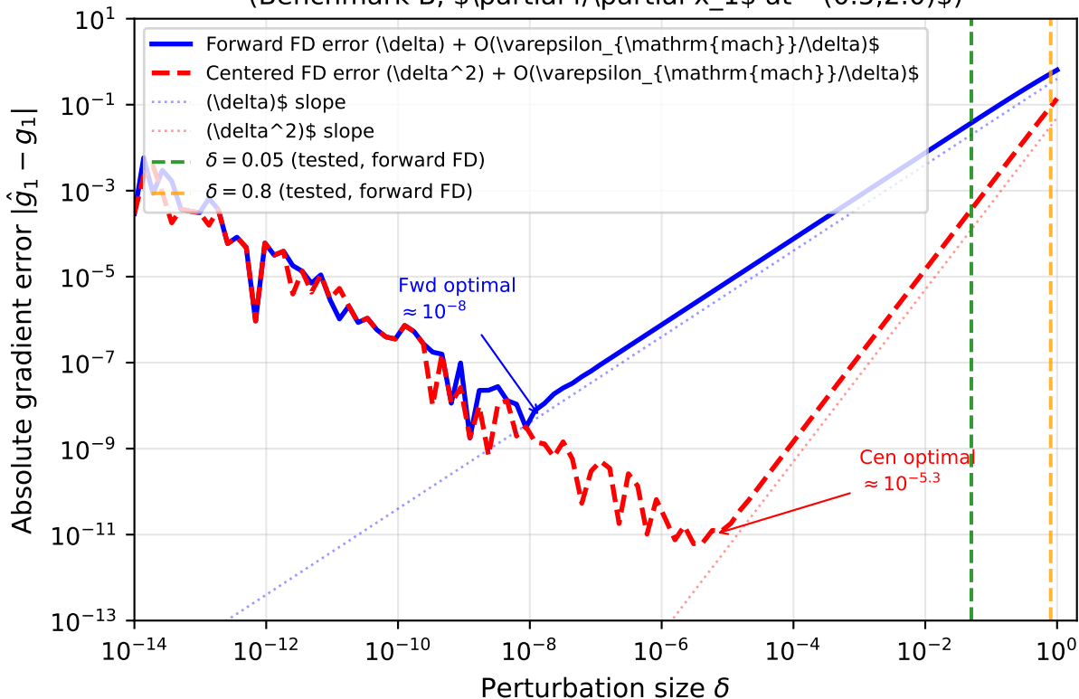
Finite Difference Gradient Error vs. Perturbation Size (Benchmark B, \partial f / \partial x_1 at (0.5, 2.0) )
