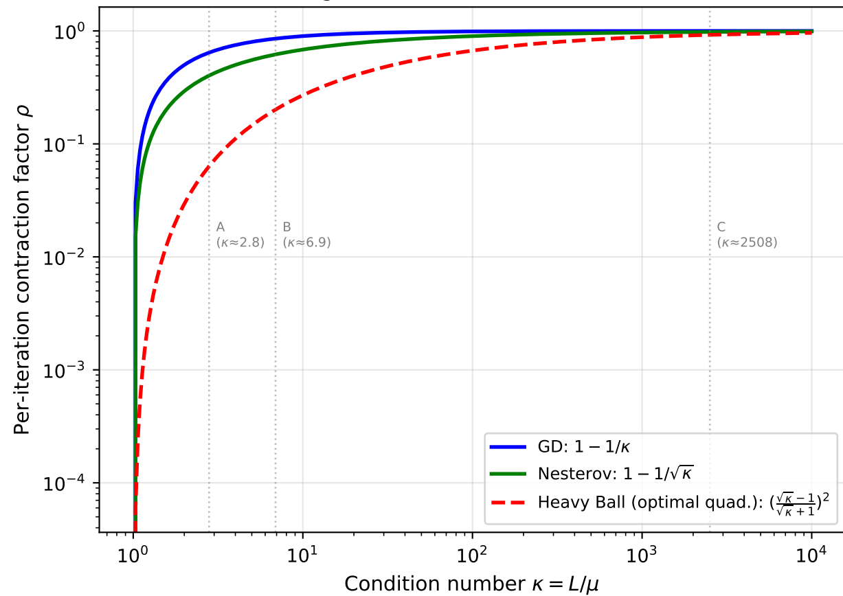
Convergence Rates vs. Condition Number
