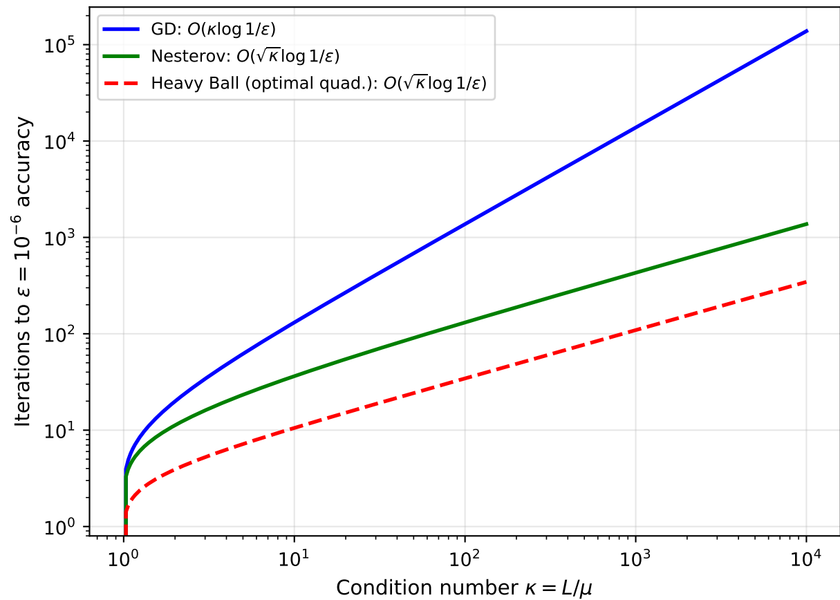
Iterations Required for \varepsilon = 10^{-6}
