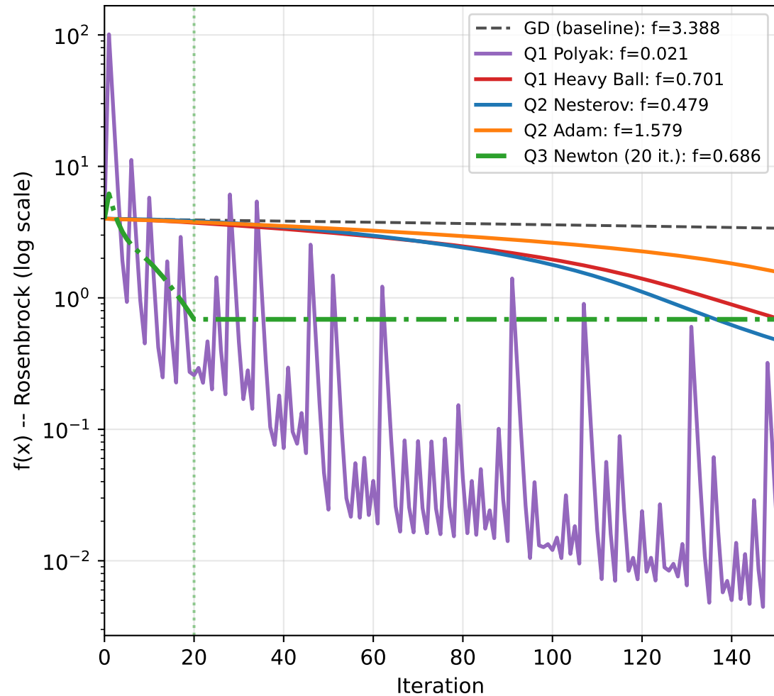
All Methods: 150 Iterations on Benchmark C
