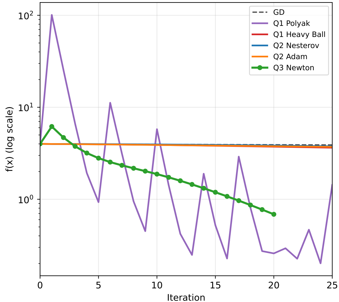
First 25 Iterations: Newton vs All
