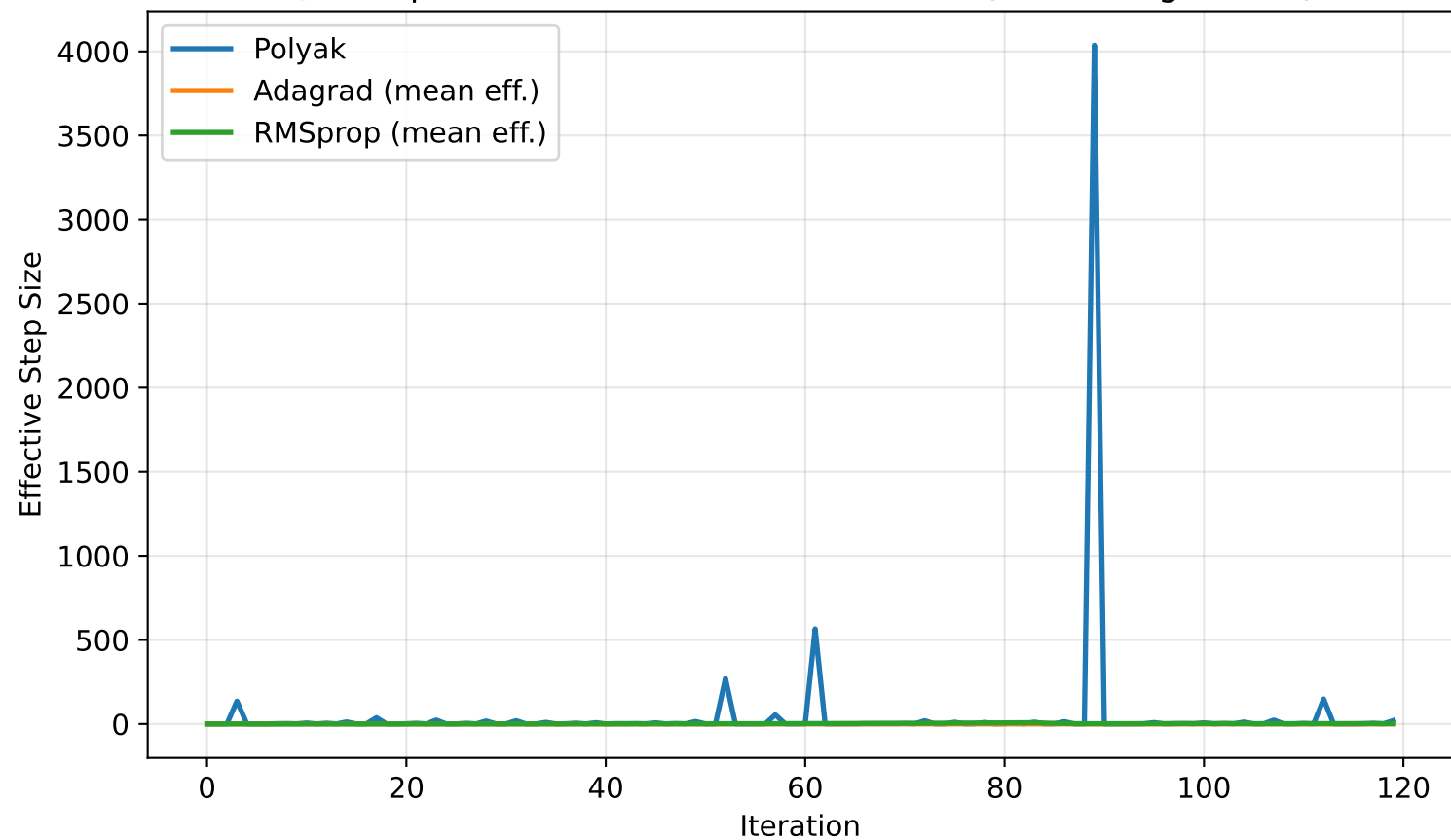
Q1: Step-Size Evolution — Benchmark A (Linear Regression)
