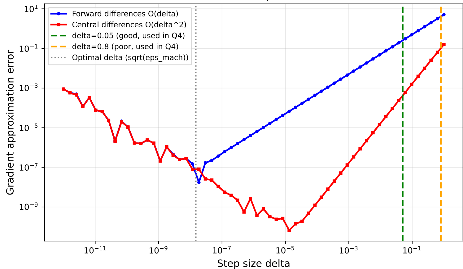
Finite Difference Gradient Error vs Step Size (Benchmark B at x=(0,3) )
