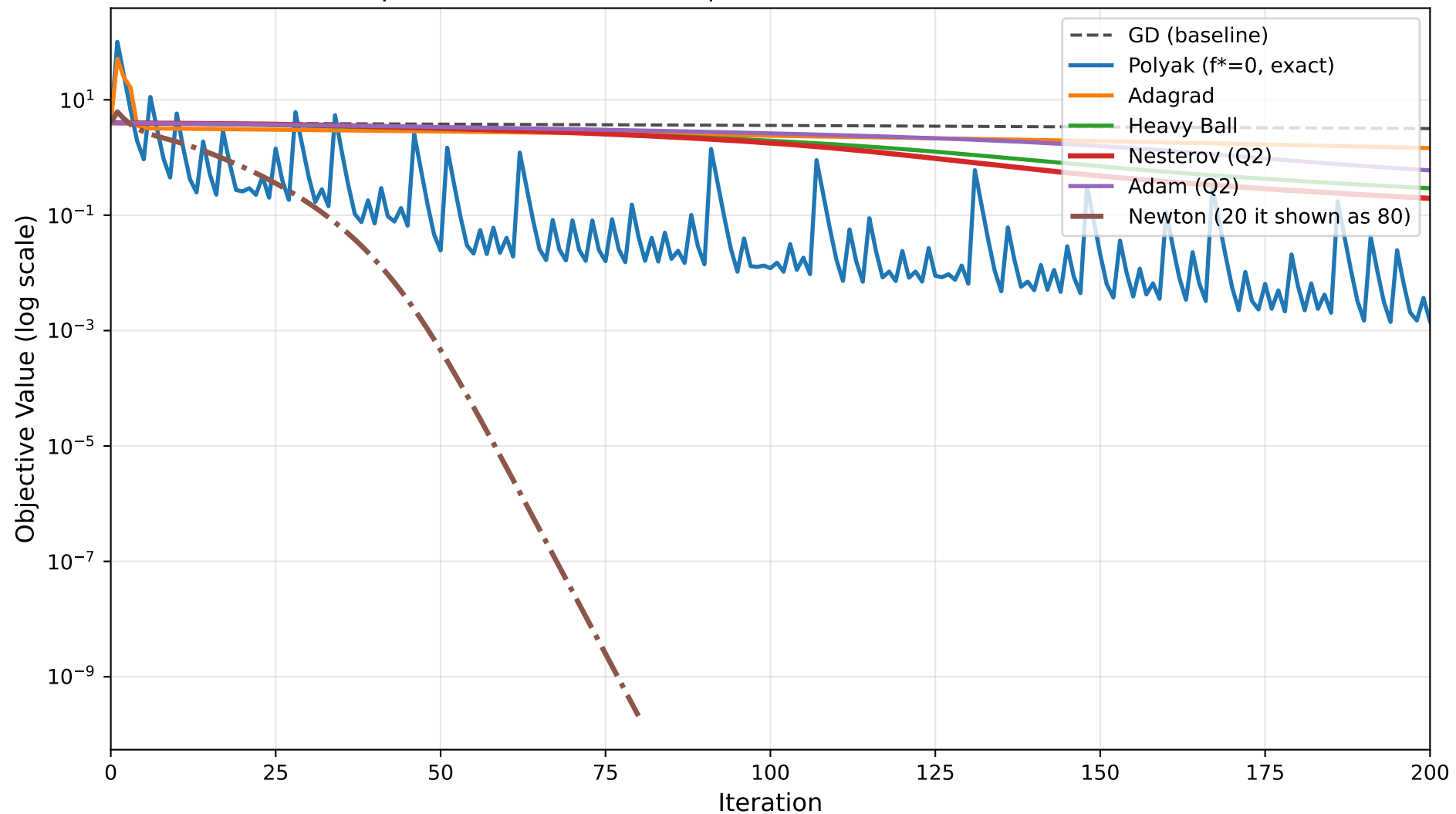
Comprehensive Method Comparison on Rosenbrock (Benchmark C)
