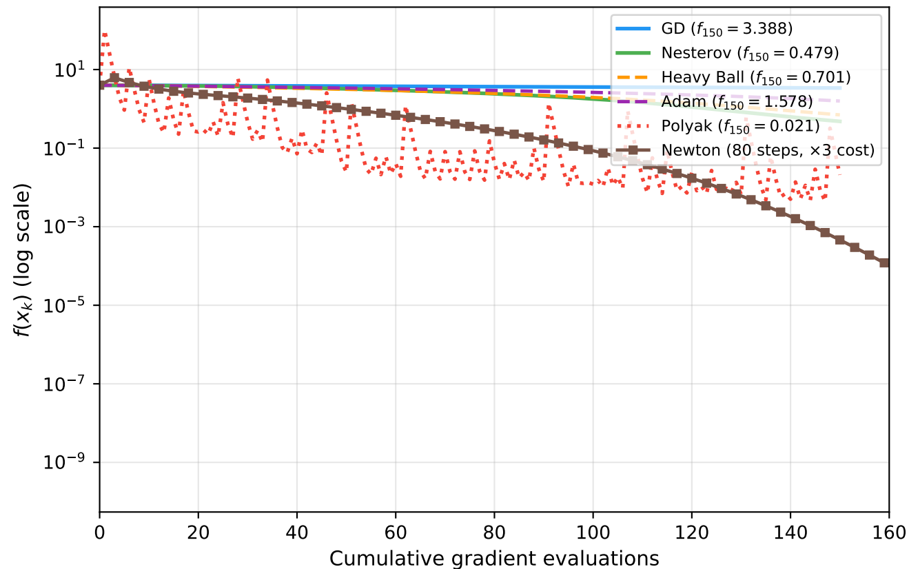
Convergence vs gradient evaluation count (Newton step = 3 grad-evals for d = 2 )
