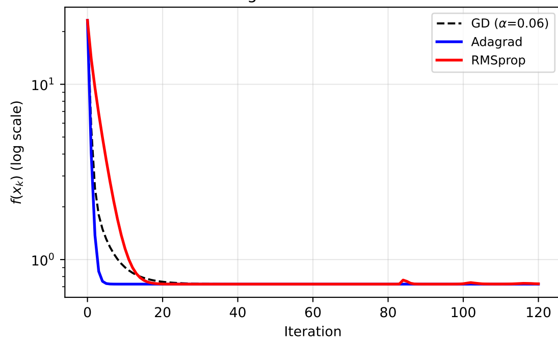
Convergence on Benchmark B
