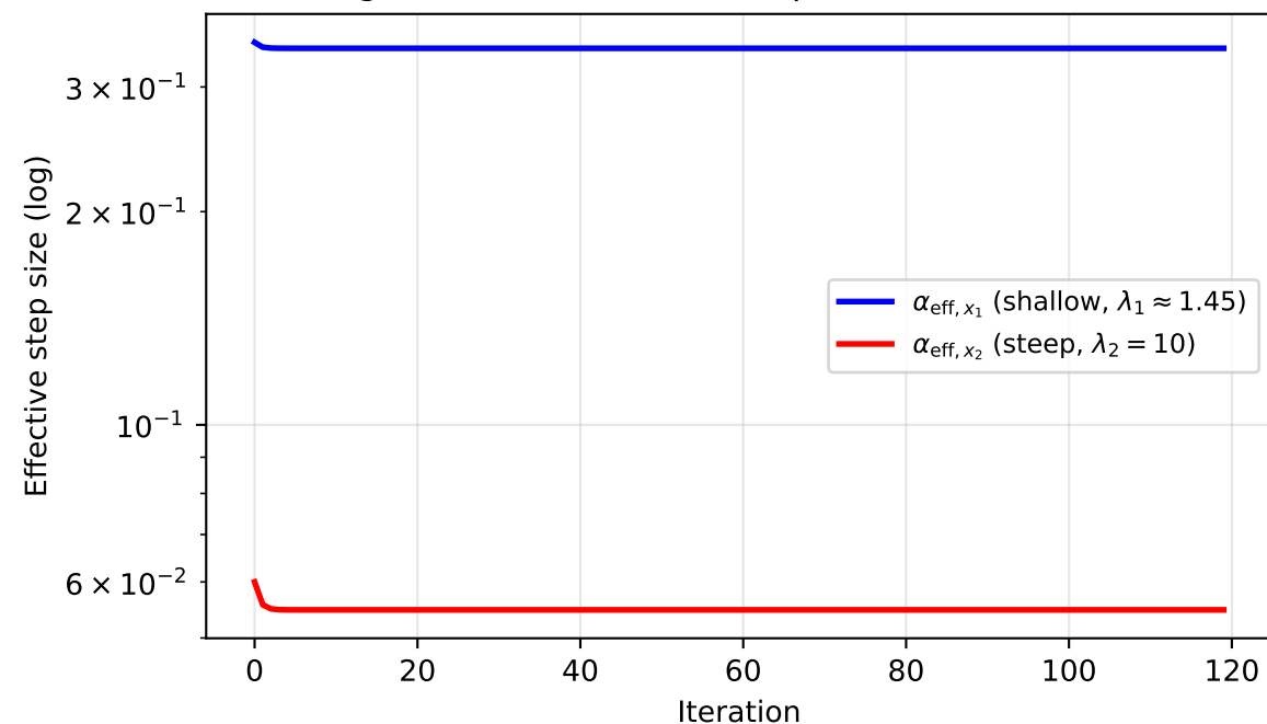
Ratio = Curvature Adaptation (ideal \approx 2.63 )
