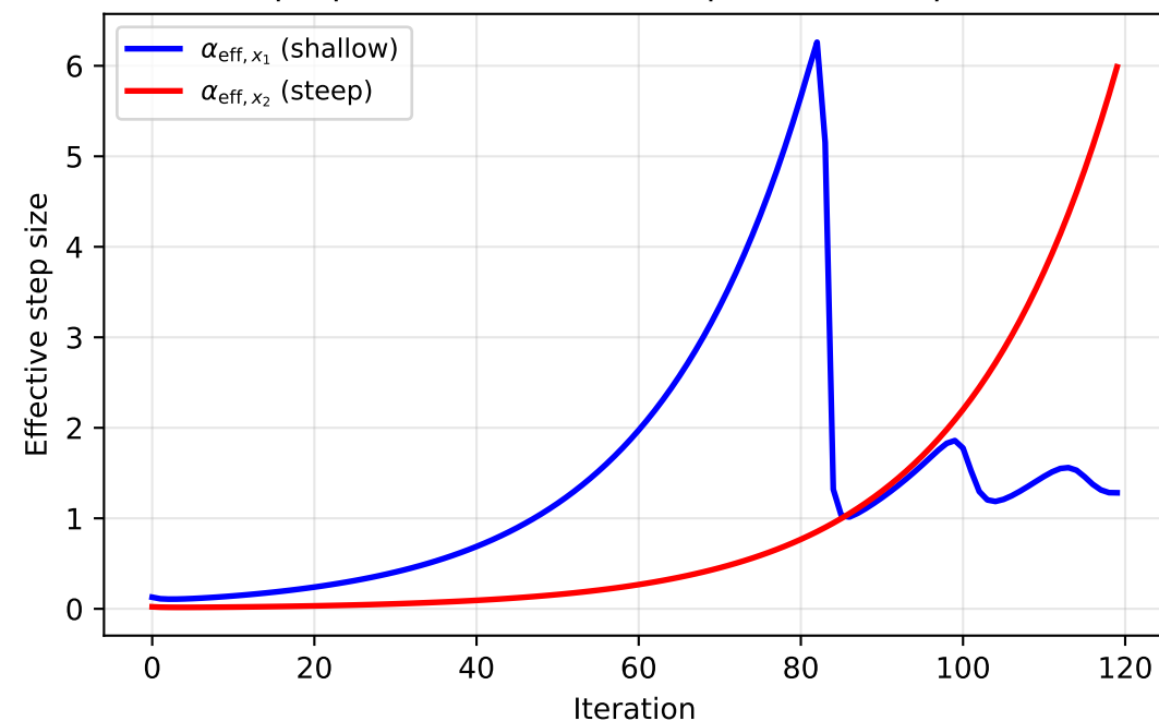
Convergence on Benchmark B
