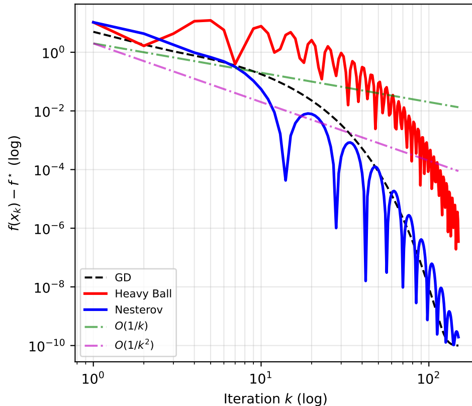
Log-Log: Convergence Rate Analysis
