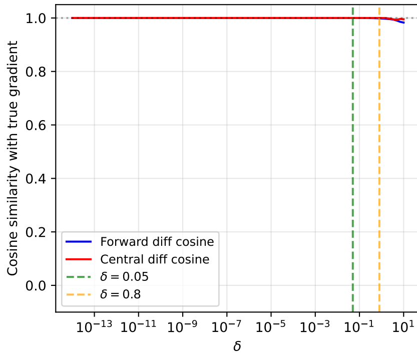
Gradient Direction Quality
