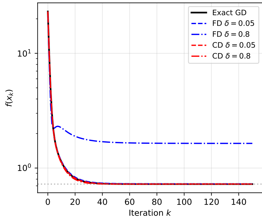
GD: FD vs CD on Benchmark B
