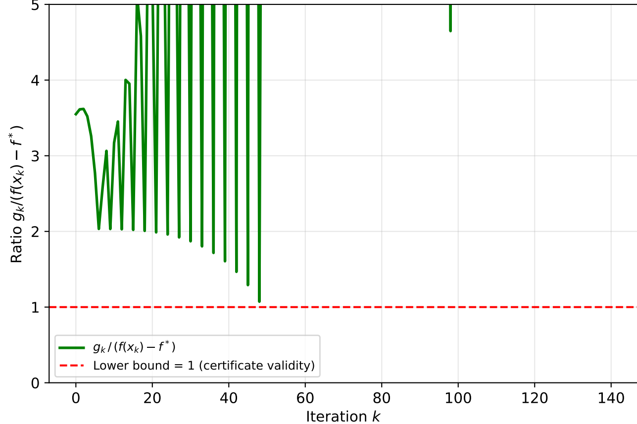
Q6: Gap g_k as Duality Certificate (ratio \geq 1 always)
