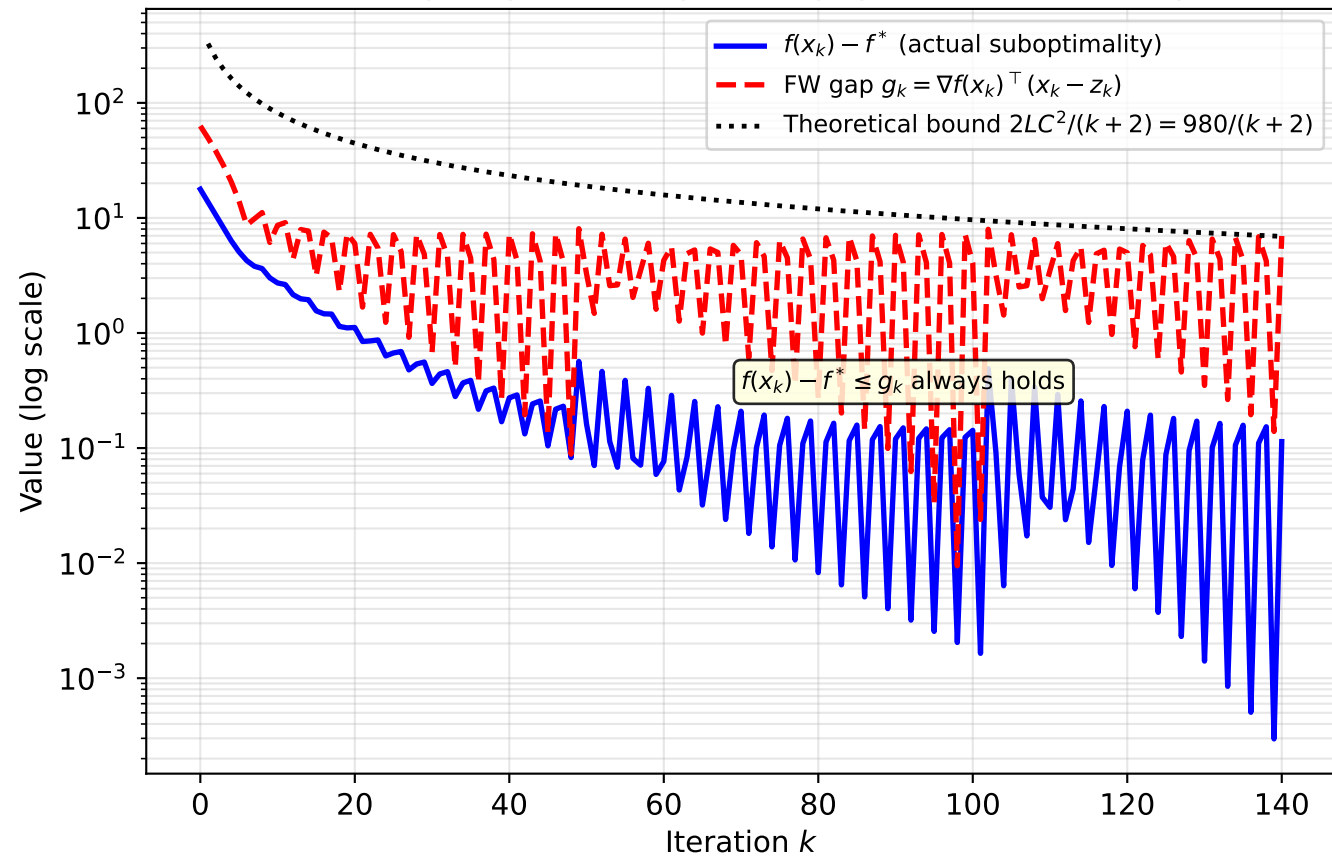
Q6: FW Duality Gap vs Suboptimality ( \beta = 0.93 , boundary case)
