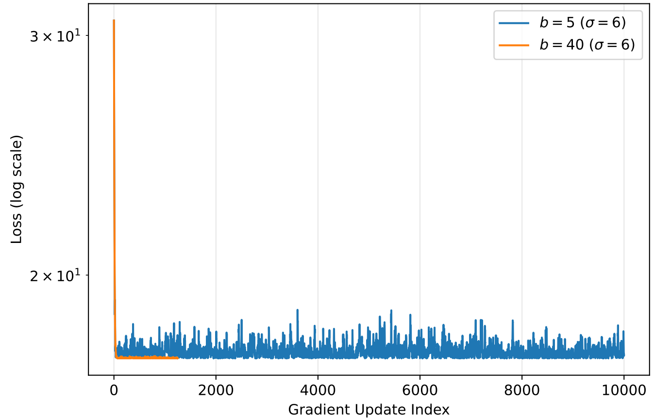
SGD: Per-Update Loss ( \sigma = 6 )
