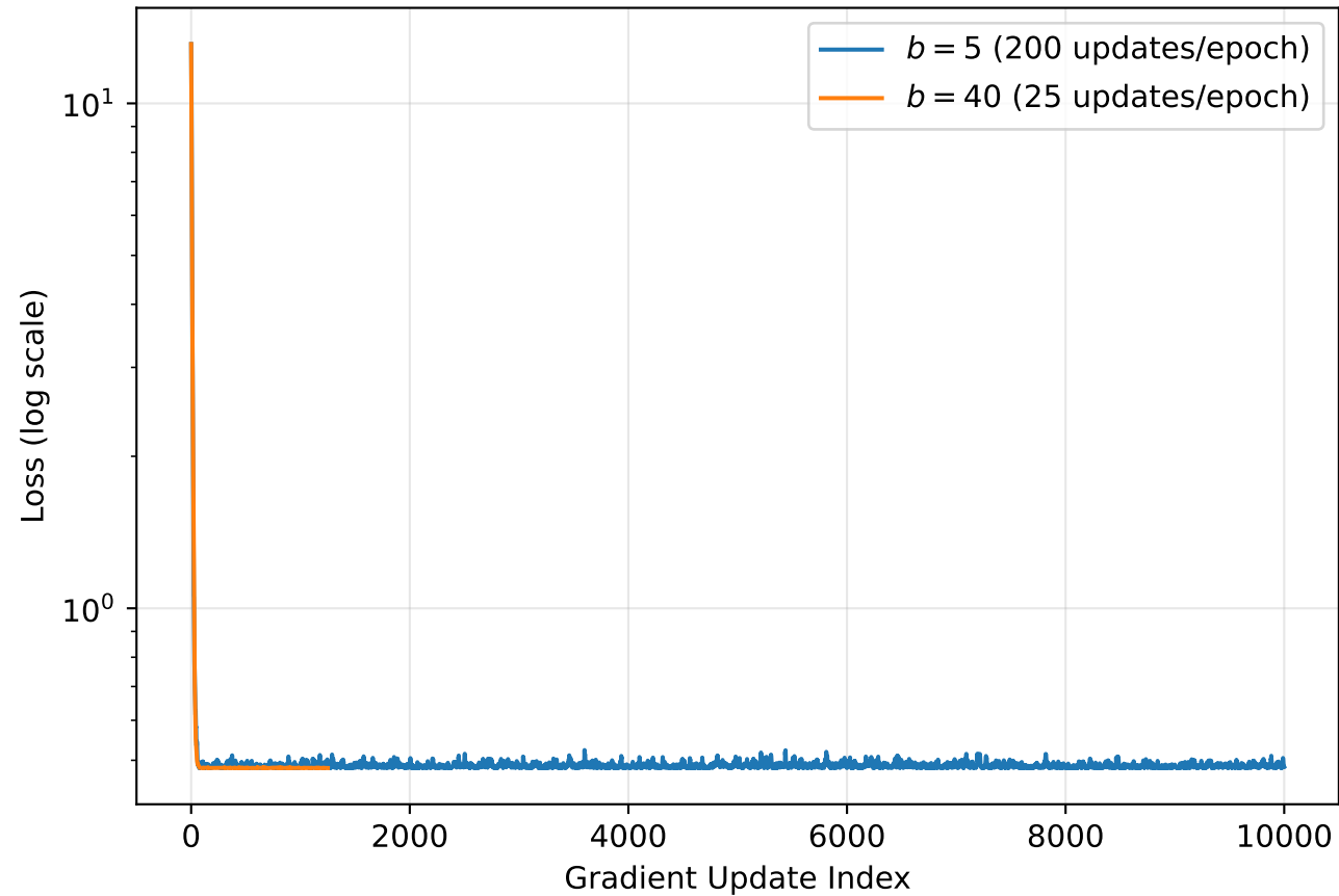
SGD: Per-Update Loss ( \sigma = 1 )
