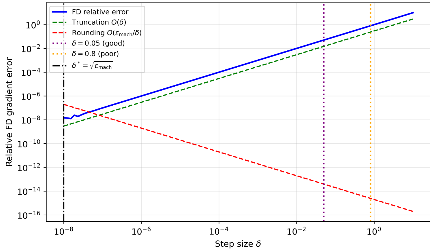
Q4: Forward FD Error vs Step Size \delta (Benchmark B, x = (0.5, 1.5) )
