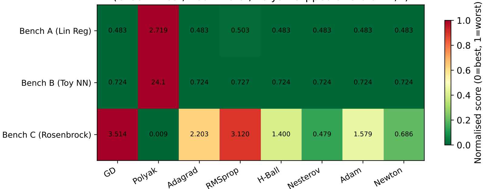
Summary: Normalised Final Objective per Method and Benchmark (Green=Best, Red=Worst; Polyak clipped at 3.0 on A,B)
