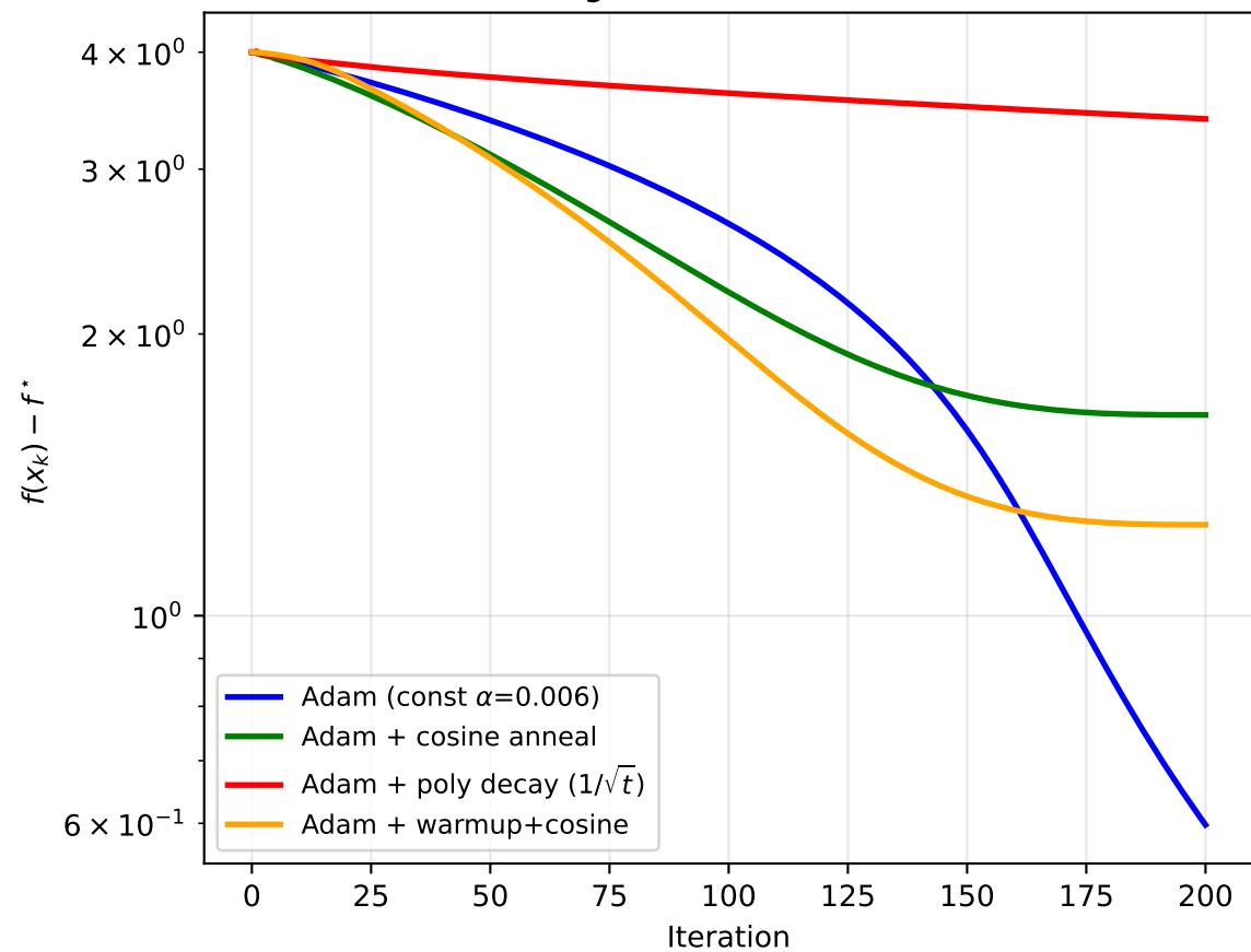
Adam: Learning Rate Schedules (Rosenbrock)
