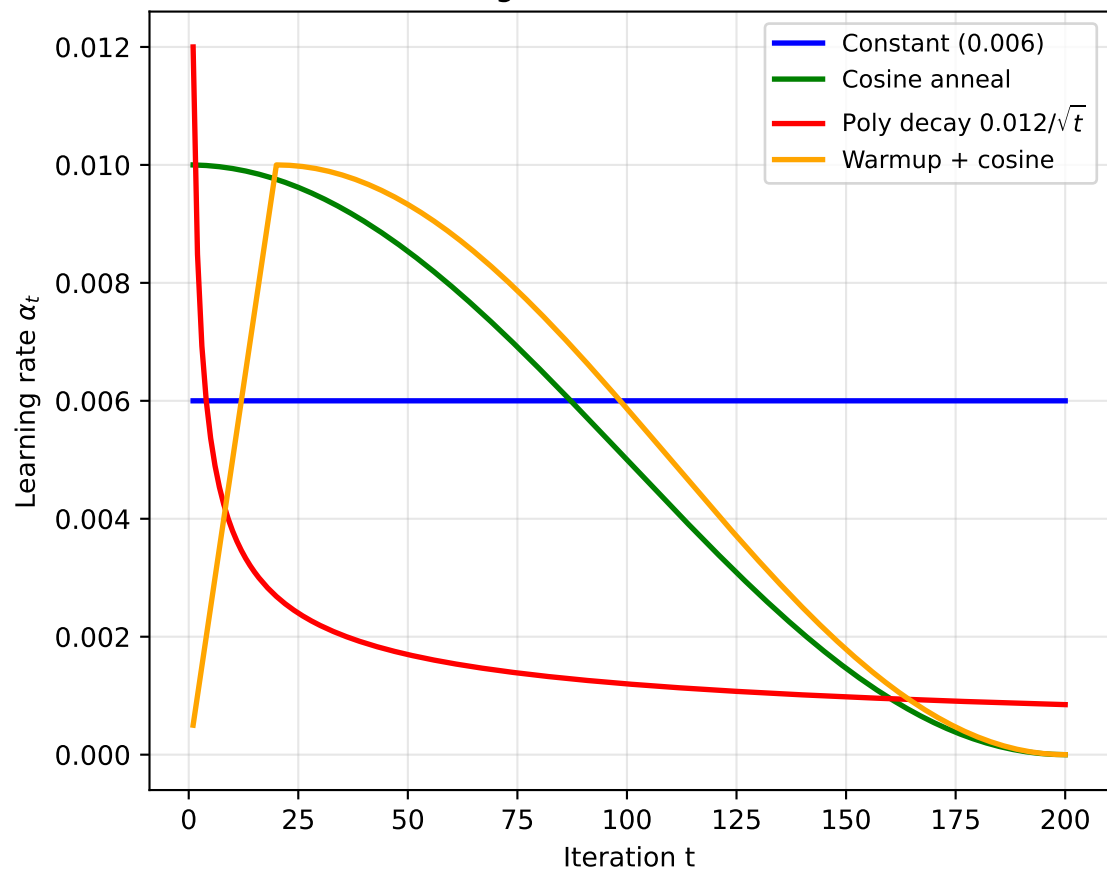
Learning Rate Schedule Profiles
