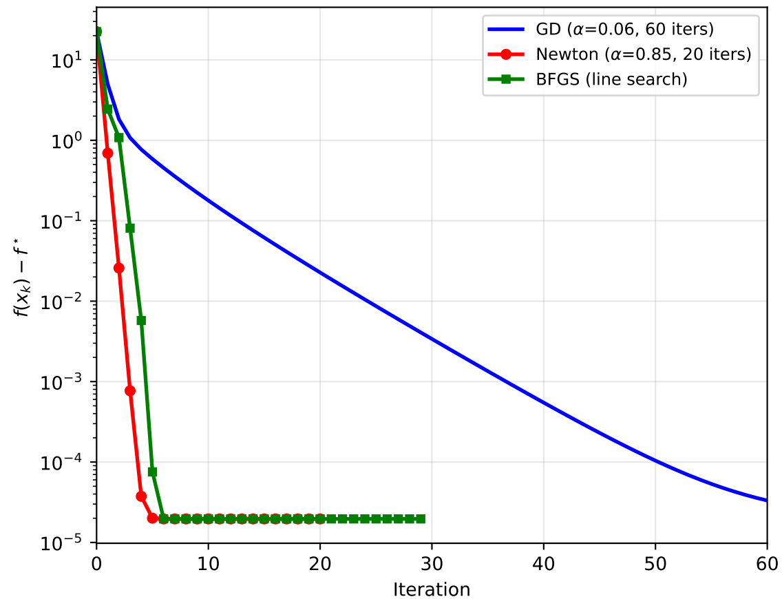
Benchmark B: GD vs Newton vs BFGS
