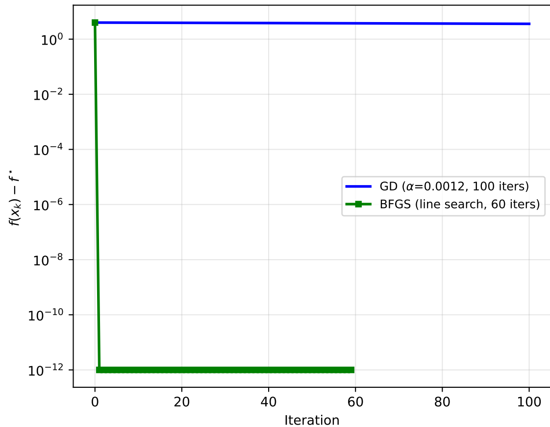
Benchmark C (Rosenbrock): GD vs BFGS
