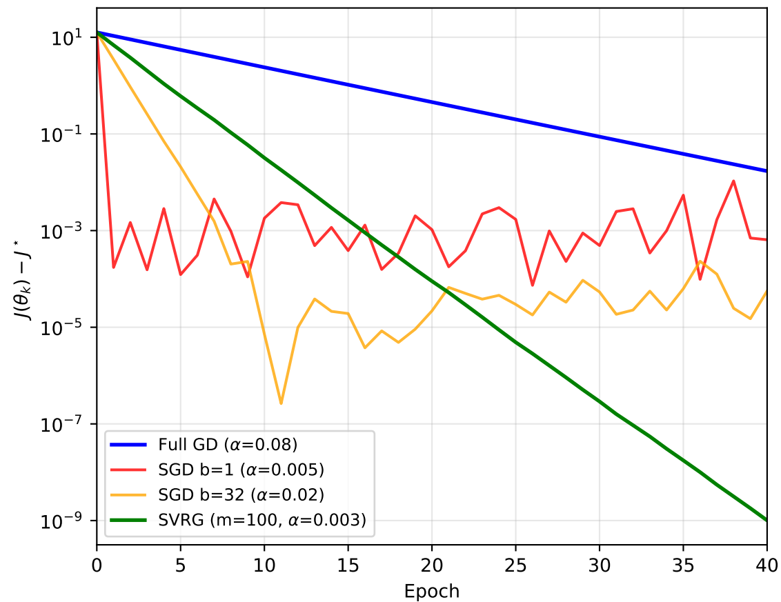
Variance Reduction: SGD vs SVRG (Benchmark A)
