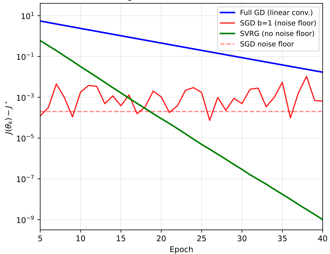
Convergence Tail: Linear vs Sublinear
