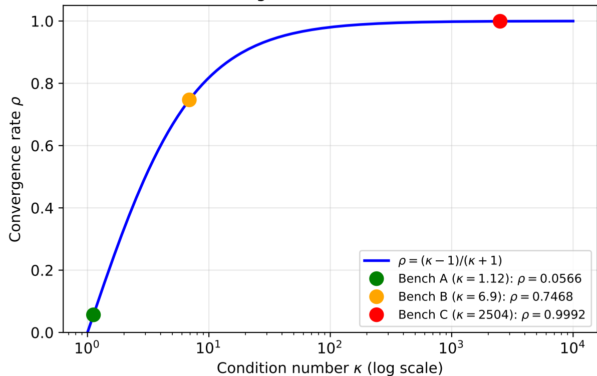
GD Linear Convergence Rate vs. Condition Number
