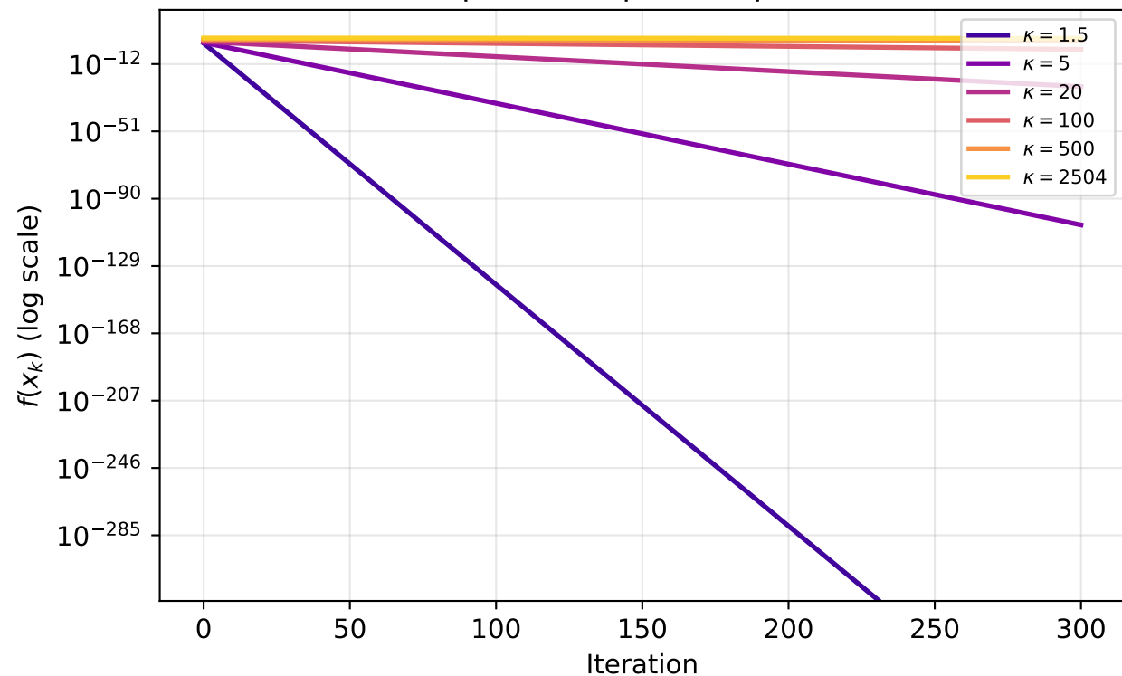
Effect of Condition Number on GD Convergence (Optimal step \alpha = 2/(\mu + L) )
