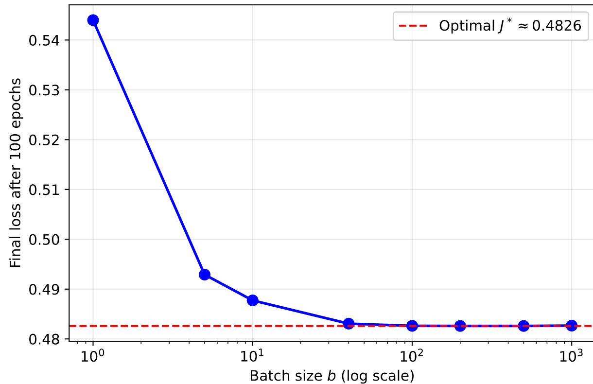
SGD Final Loss vs. Batch Size (Benchmark A)
