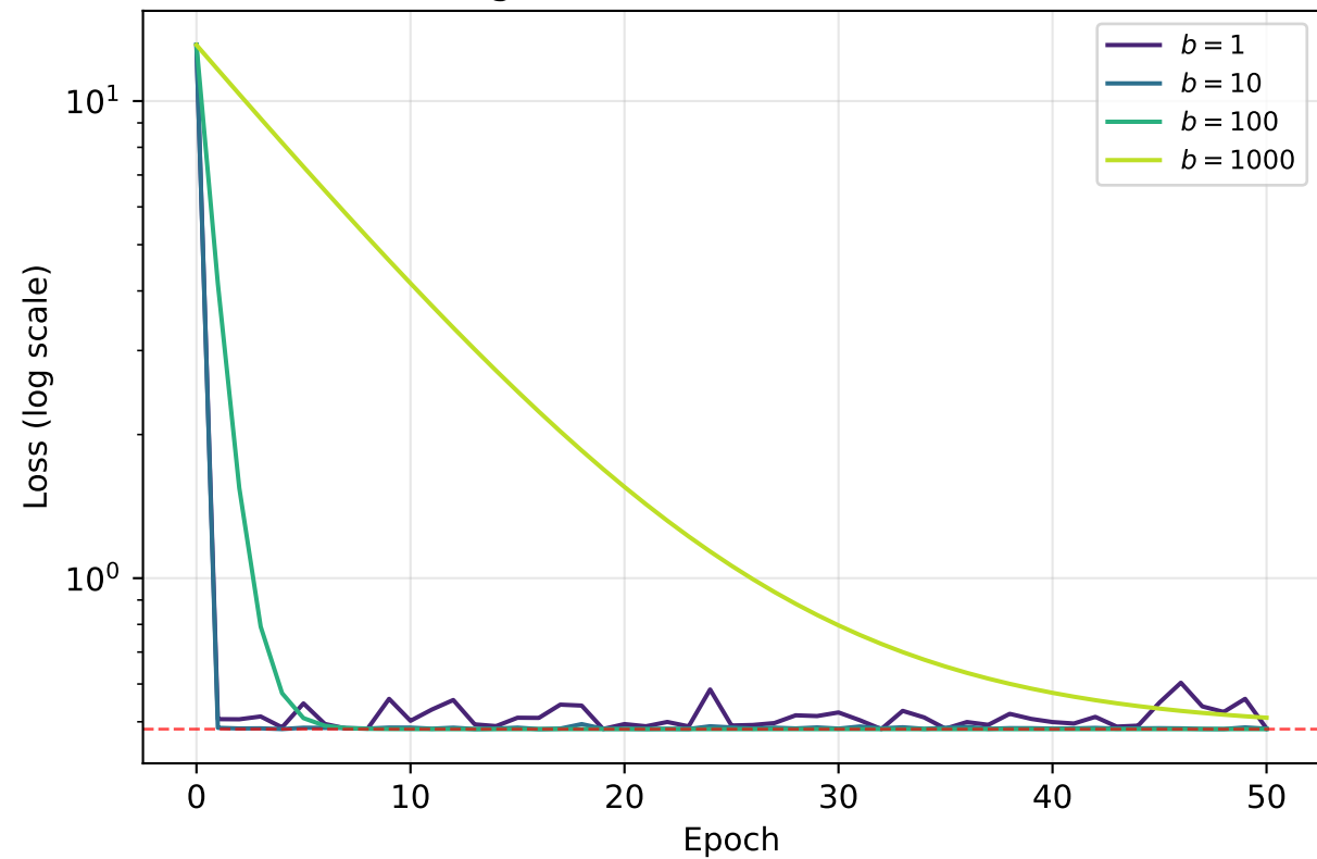
SGD Convergence Curves for Various Batch Sizes
