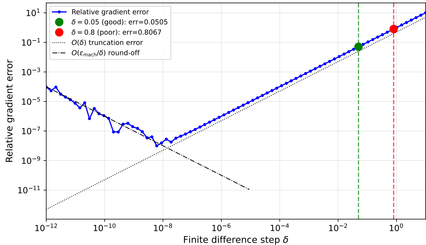
Q4: Finite Difference Gradient Error vs. Step Size \delta (Benchmark B)
