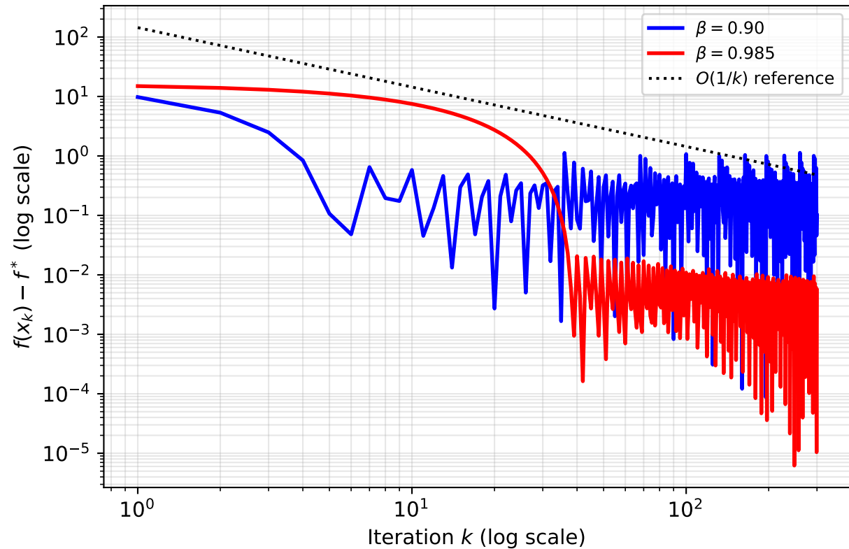
Q6: Frank--Wolfe Convergence on Log-Log Scale
