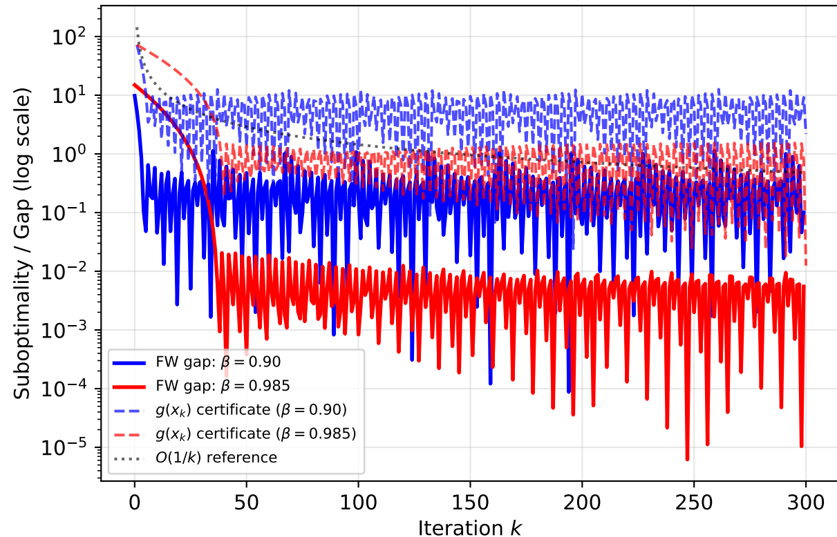
Q6: Frank--Wolfe Gap Certificate g(x_k) \geq f(x_k) - f^*
