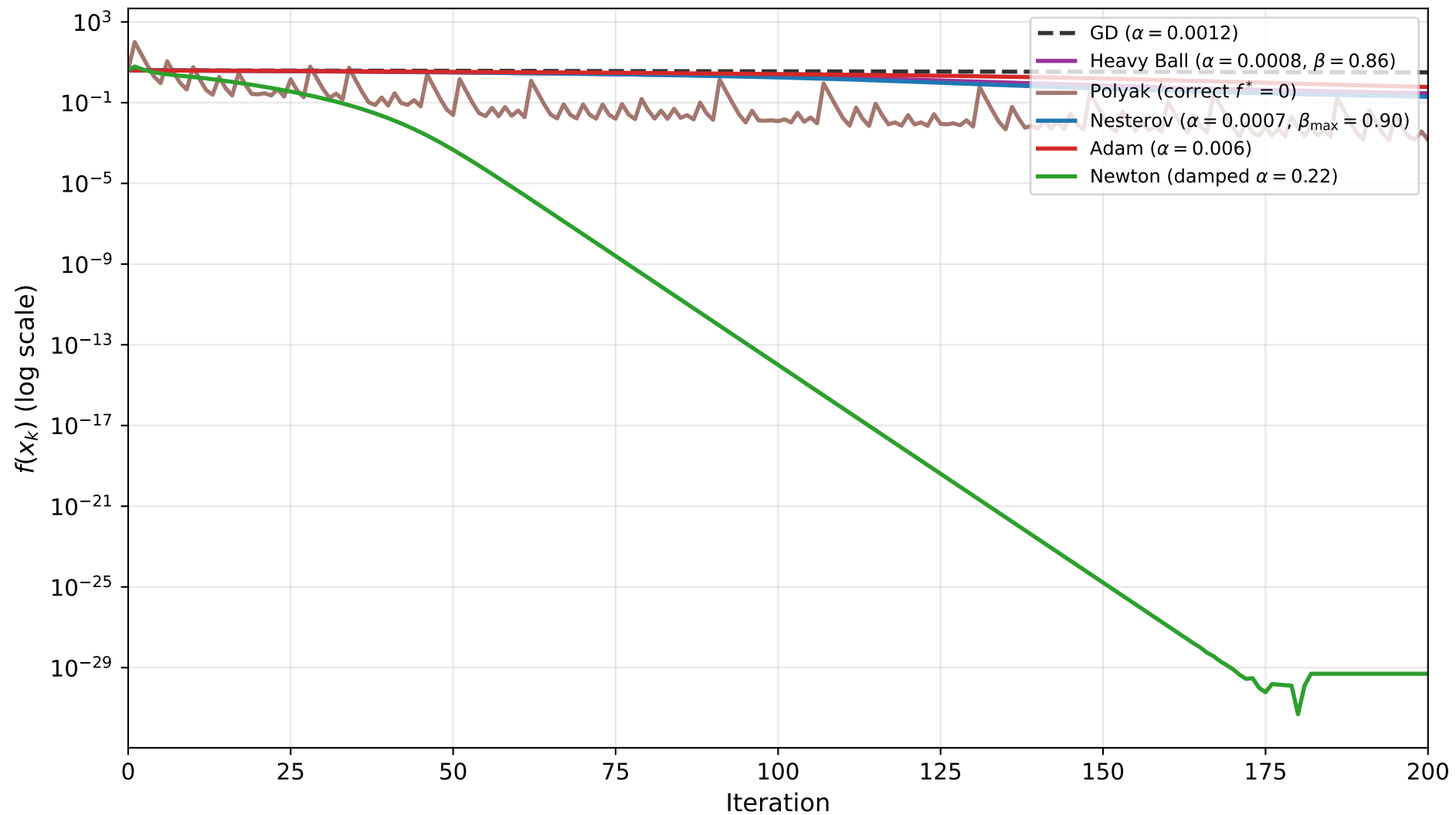
Summary: All Best Methods on Benchmark C (Rosenbrock, \kappa \approx 2504 )
